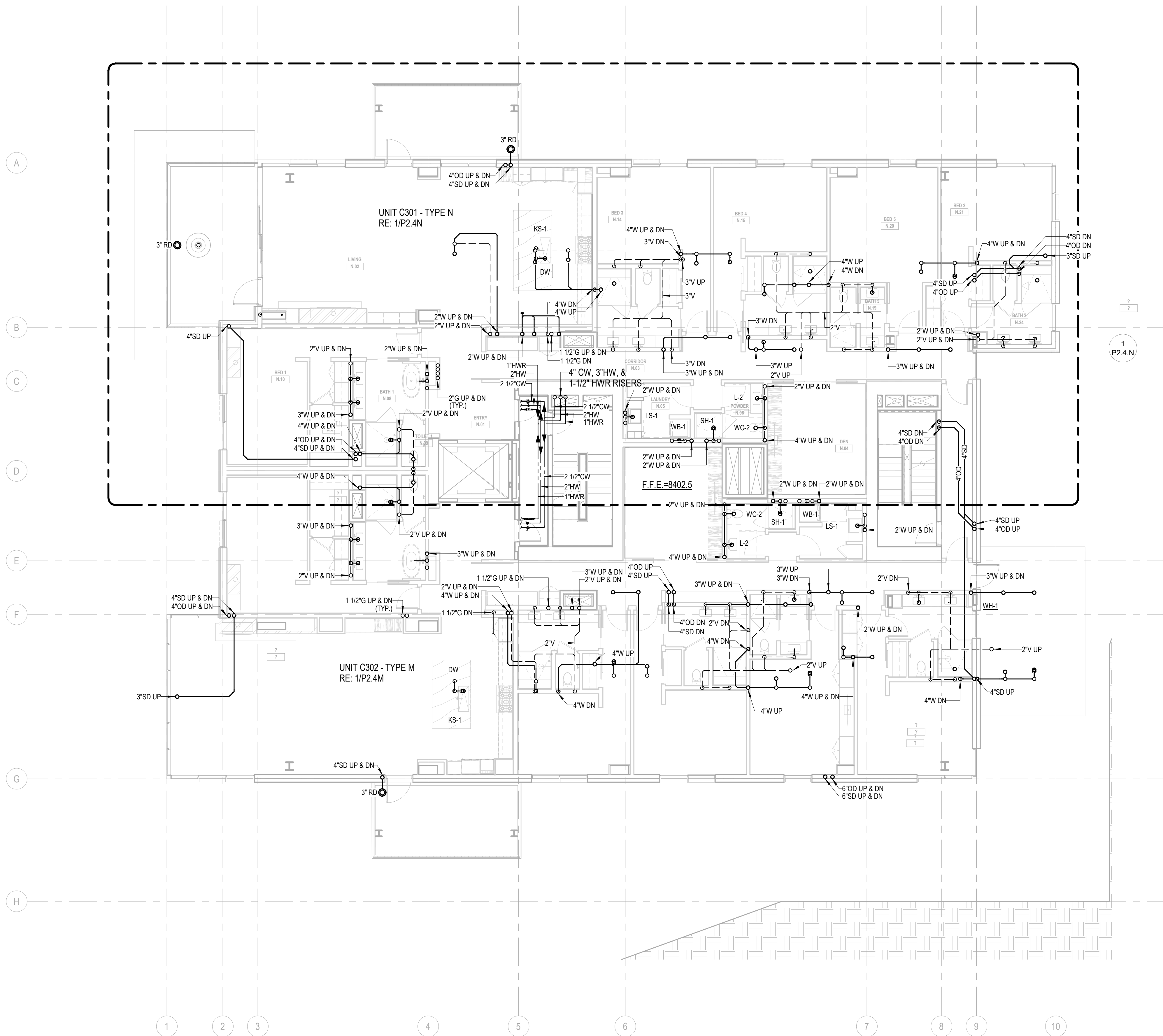
1 PLAN - TOWER C - LVL 3 SCALE: 1/8" = 1'-0"
