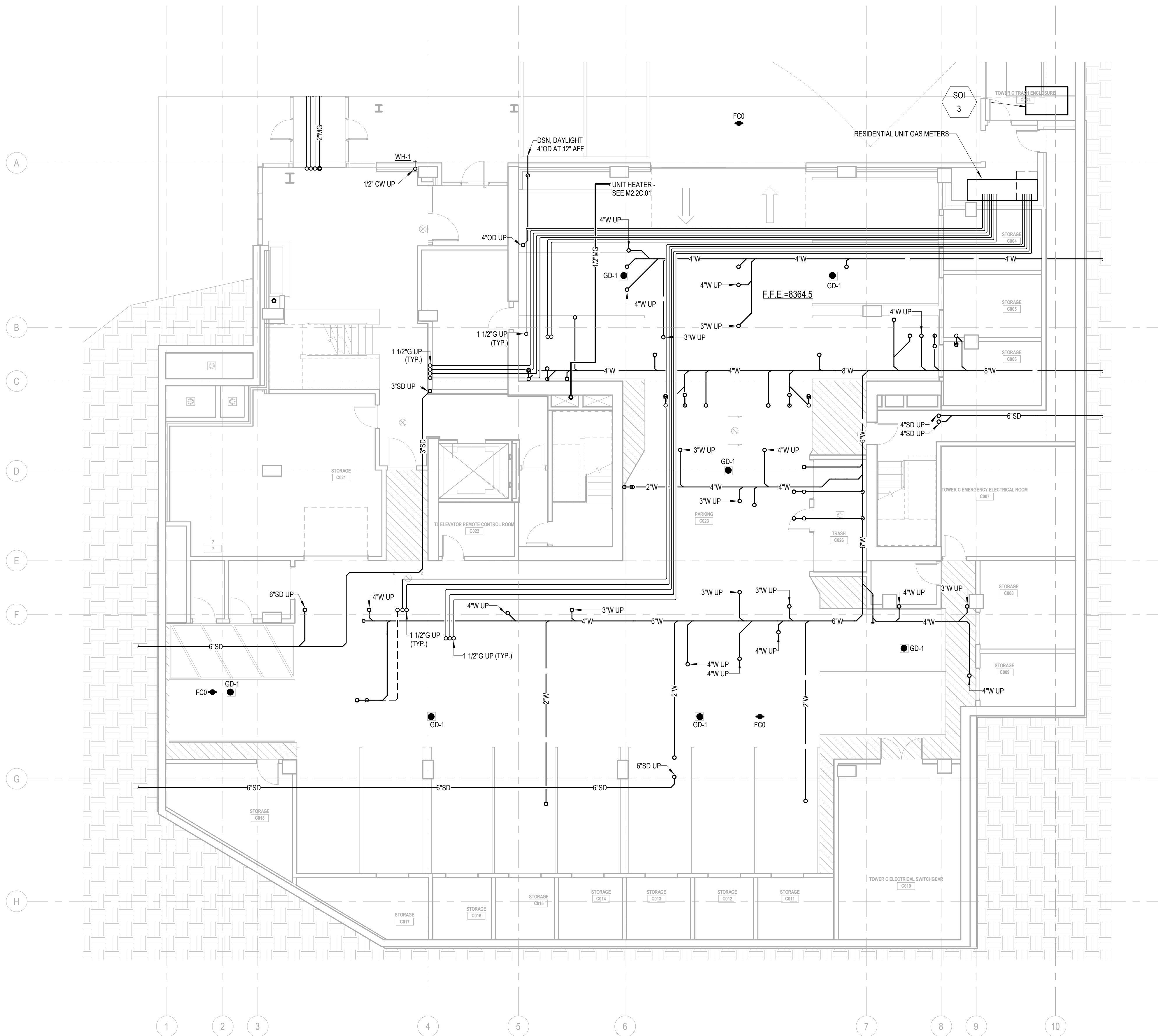
1 PLAN - TOWER C - LVL P1 SCALE: 1/8" = 1'-0"
