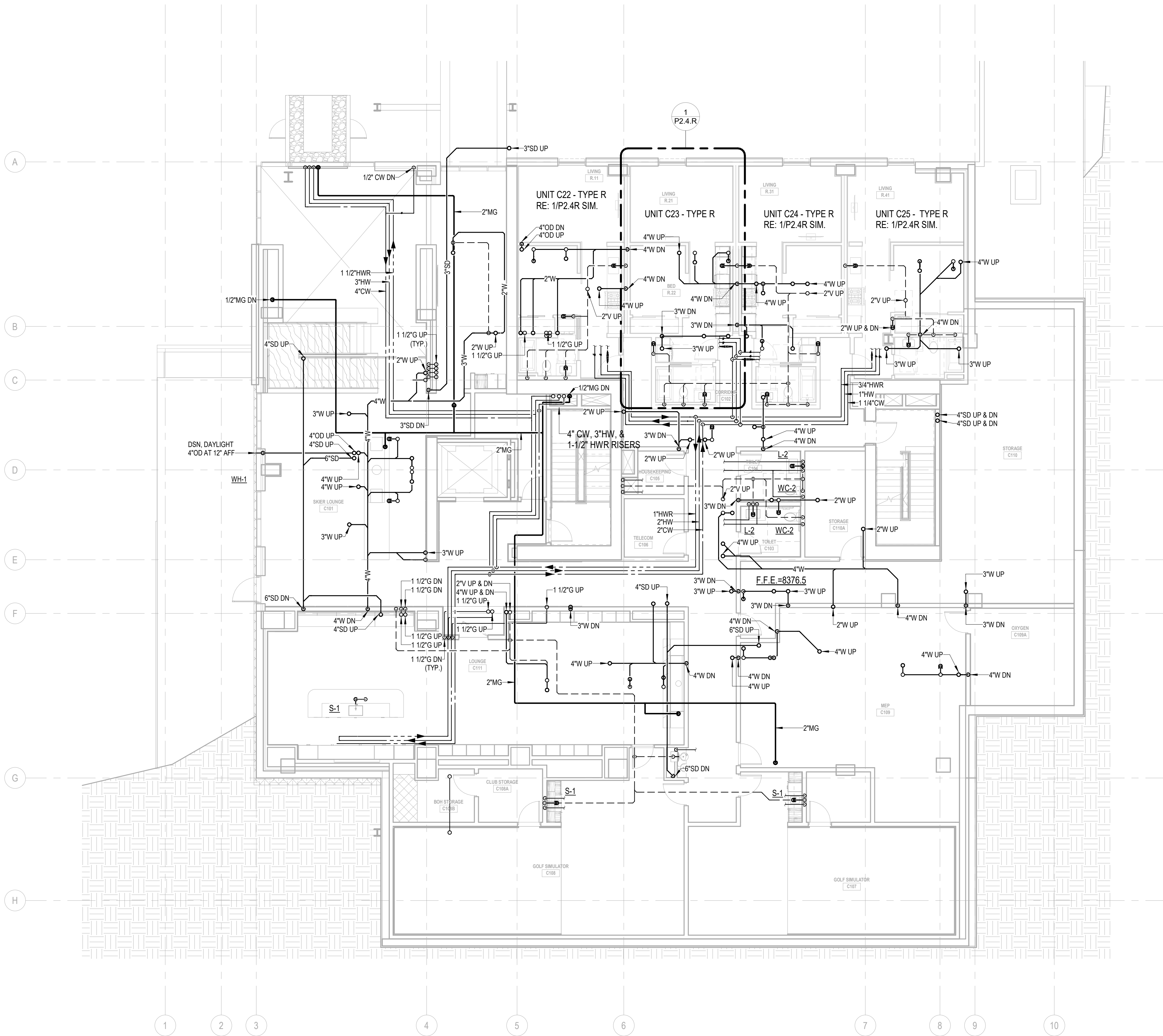
1 PLAN - TOWER C - LVL 1 SCALE: 1/8" = 1'-0"
