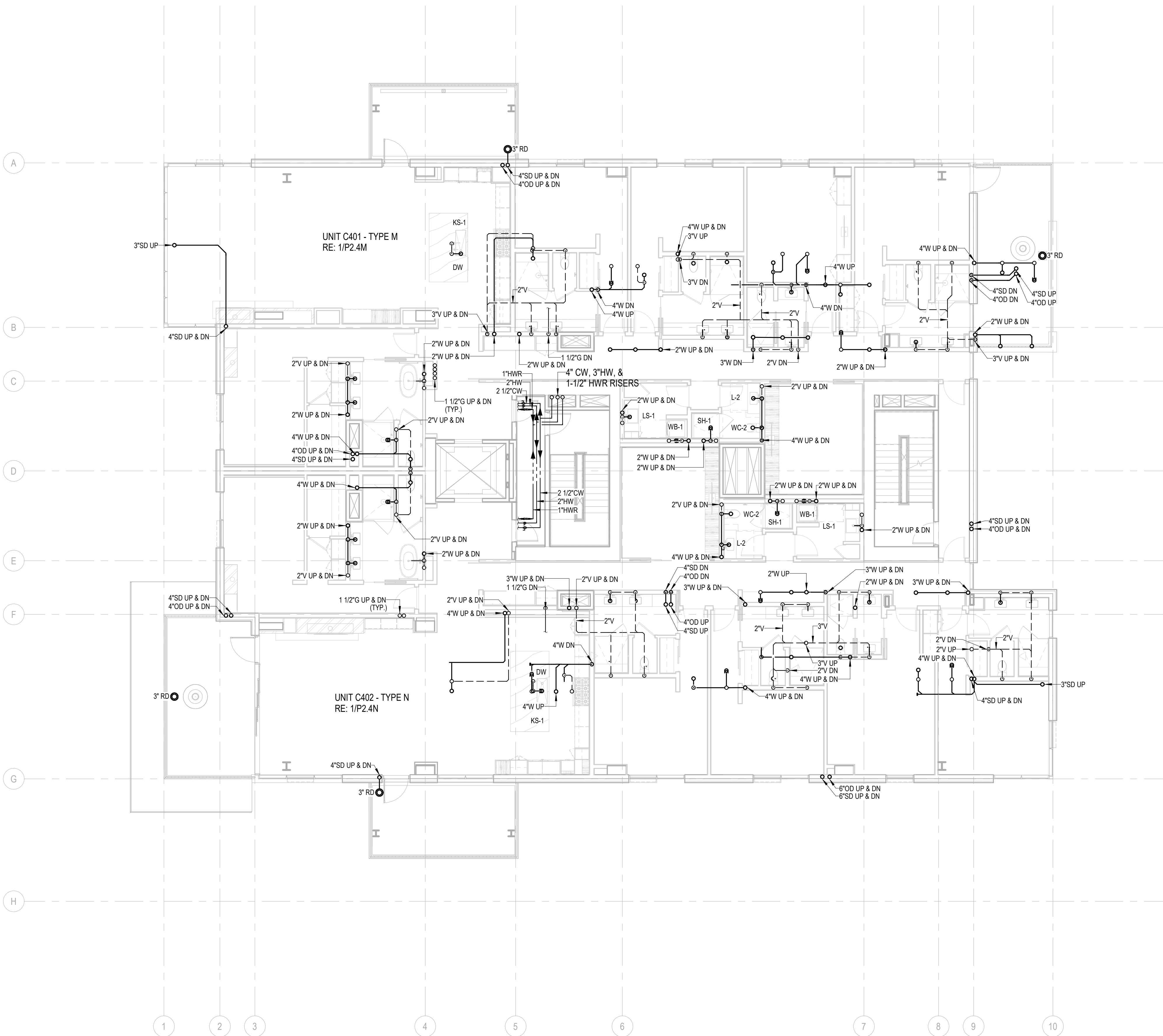
1 PLAN - TOWER C - LVL 4 SCALE: 1/8" = 1'-0"
