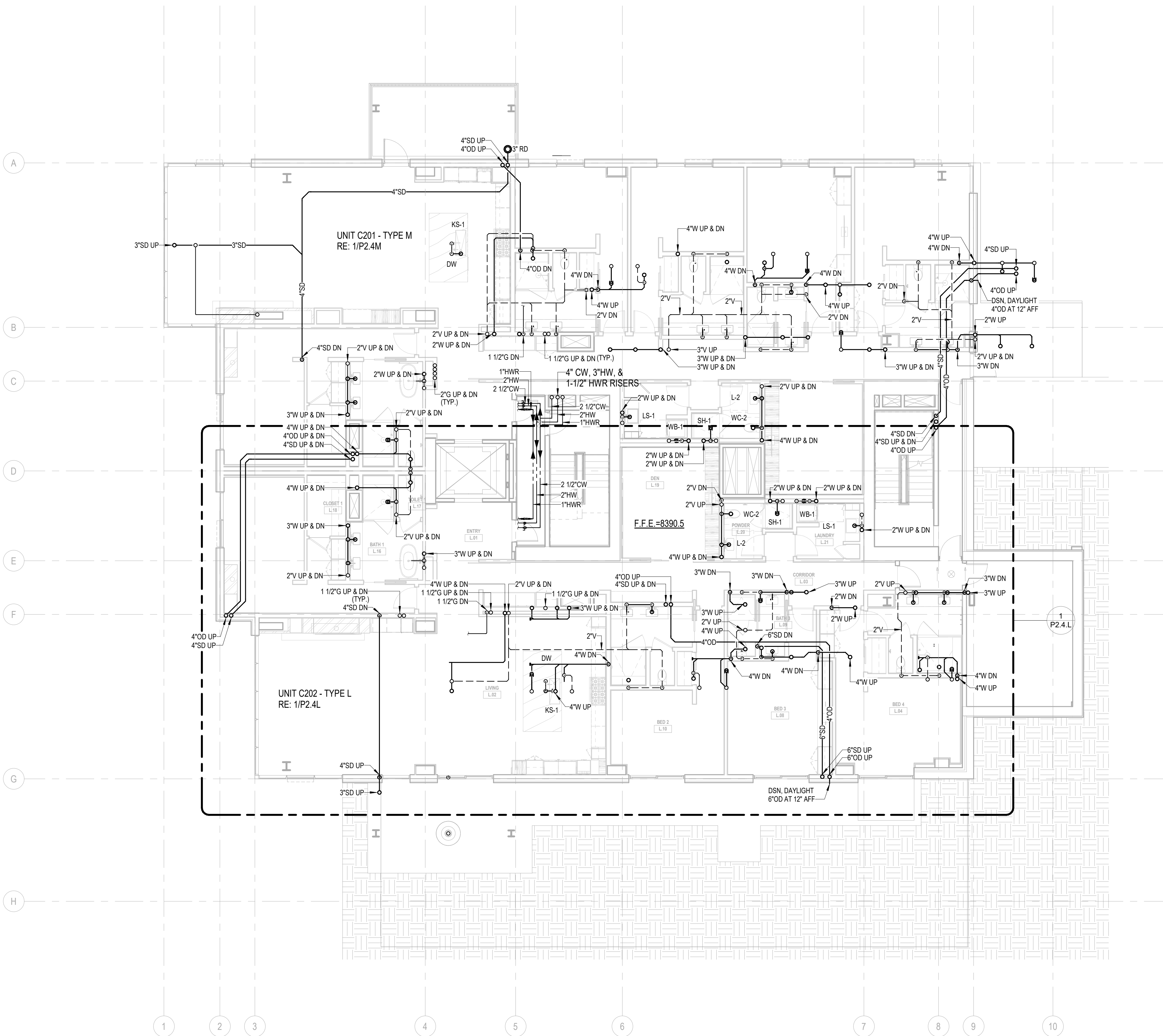
1 PLAN - TOWER C - LVL 2 SCALE: 1/8" = 1'-0"
