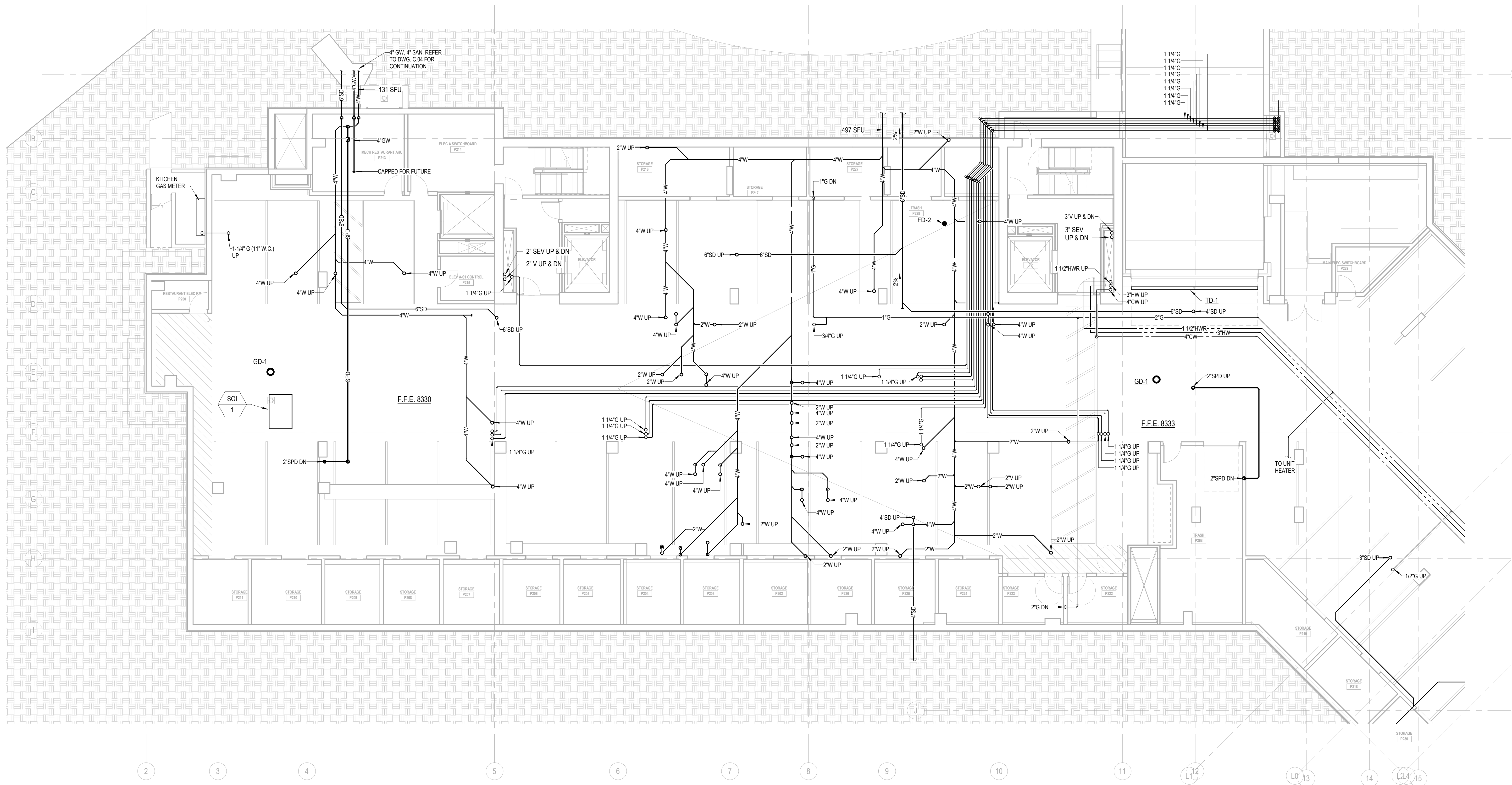
1 PLAN - TOWER A - LVL P2 SCALE: 1/8" = 1'-0"
