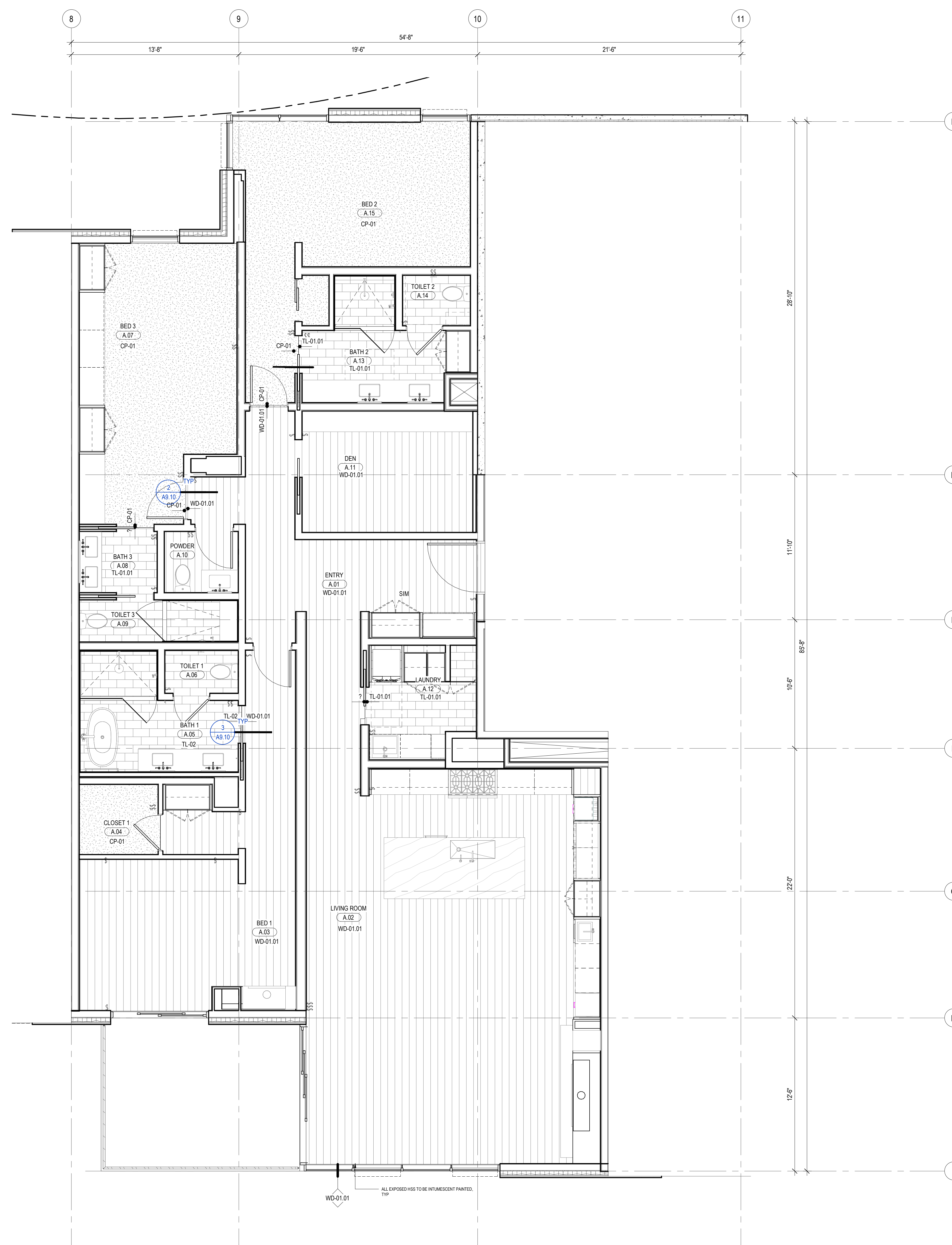
1 FINISH PLAN - TOWER A/B - UNIT A SCALE: 1/4" = 1'-0"
