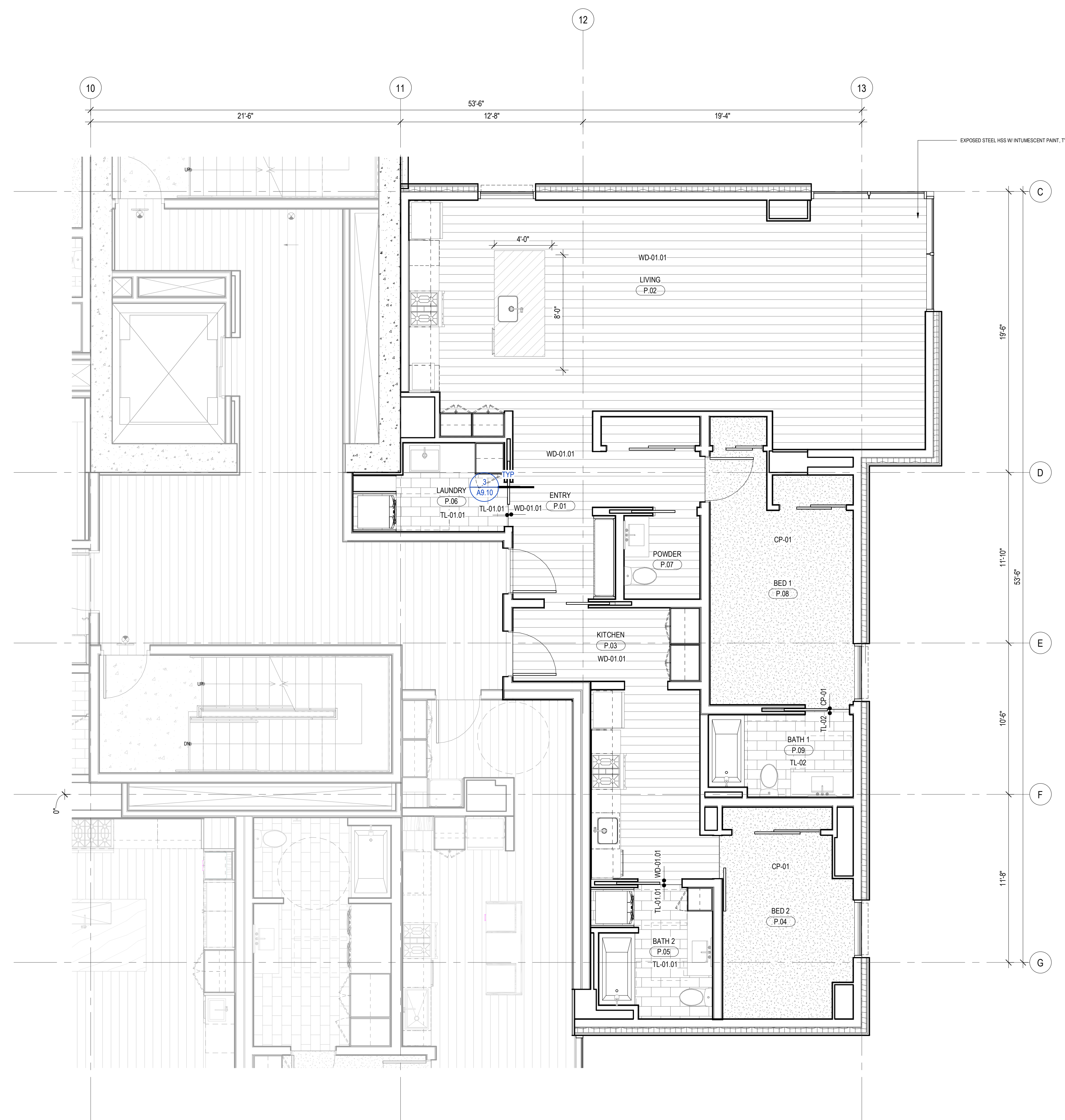
1 FINISH PLAN - TOWER A/B - UNIT P SCALE: 1/4" = 1'-0"
