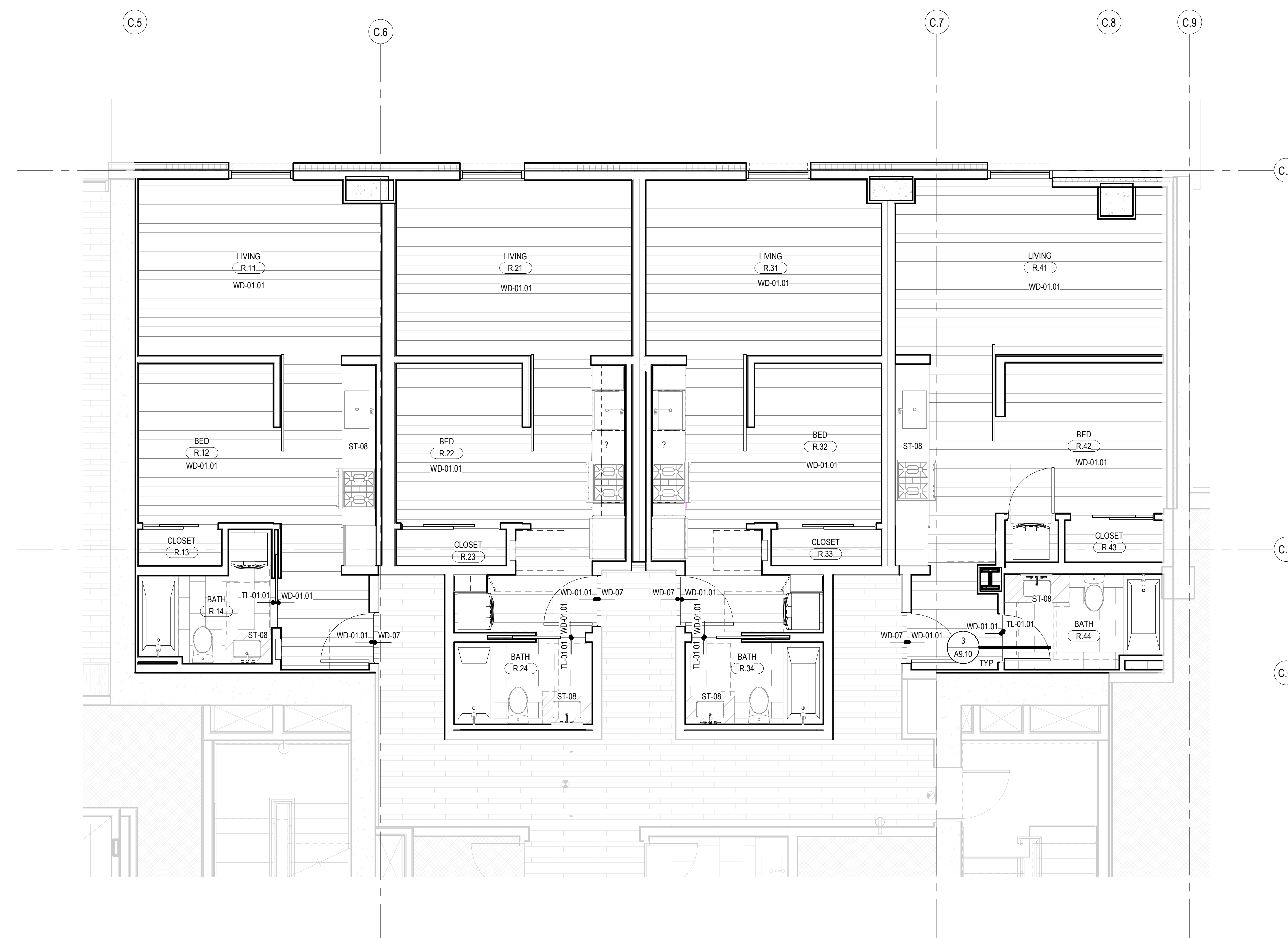
1 FINISH PLAN - TOWER C - UNIT R SCALE: 1/4" = 1'-0"
