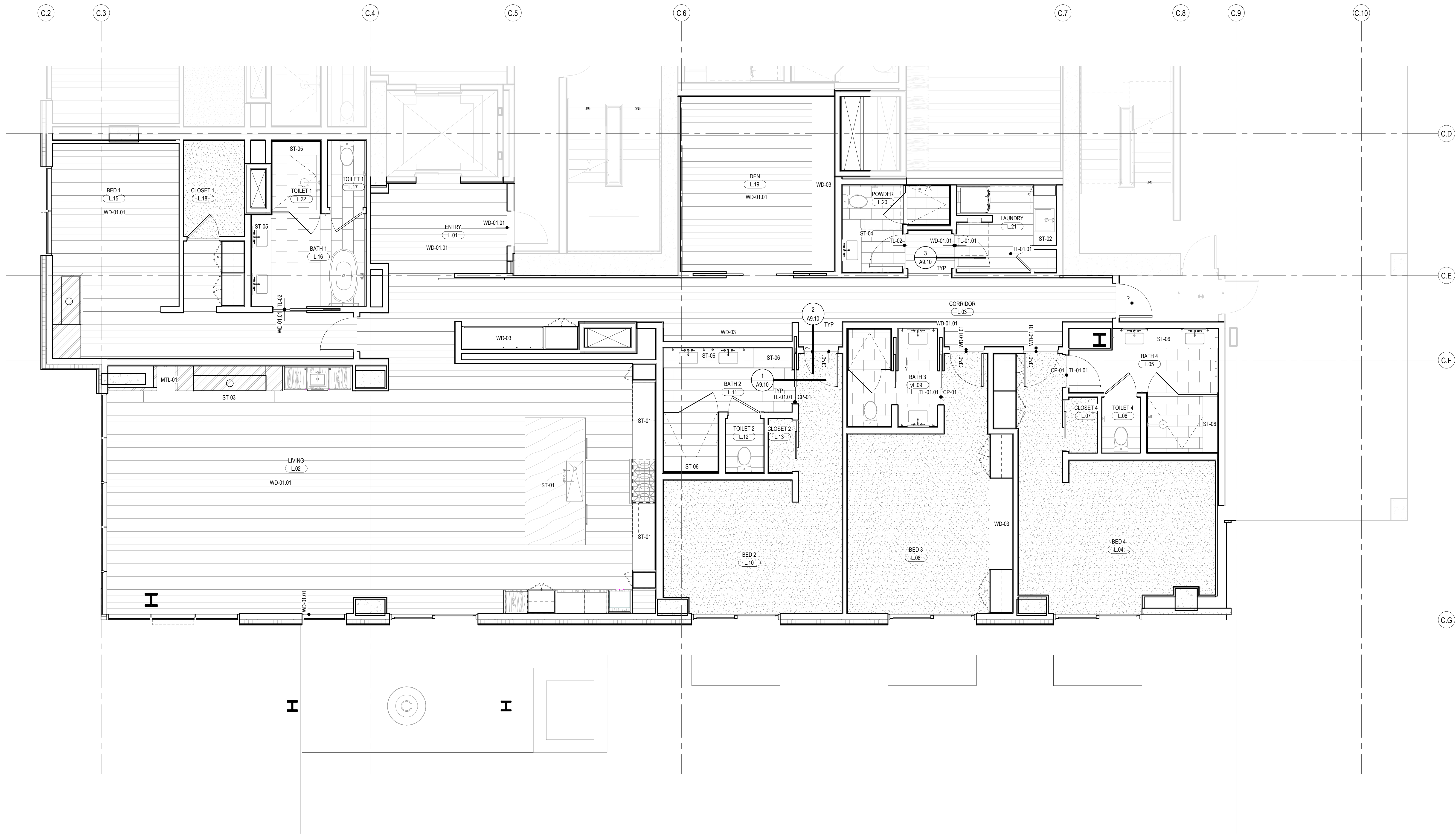
1 FINISH PLAN - TOWER C - UNIT L SCALE: 1/4" = 1'-0"
