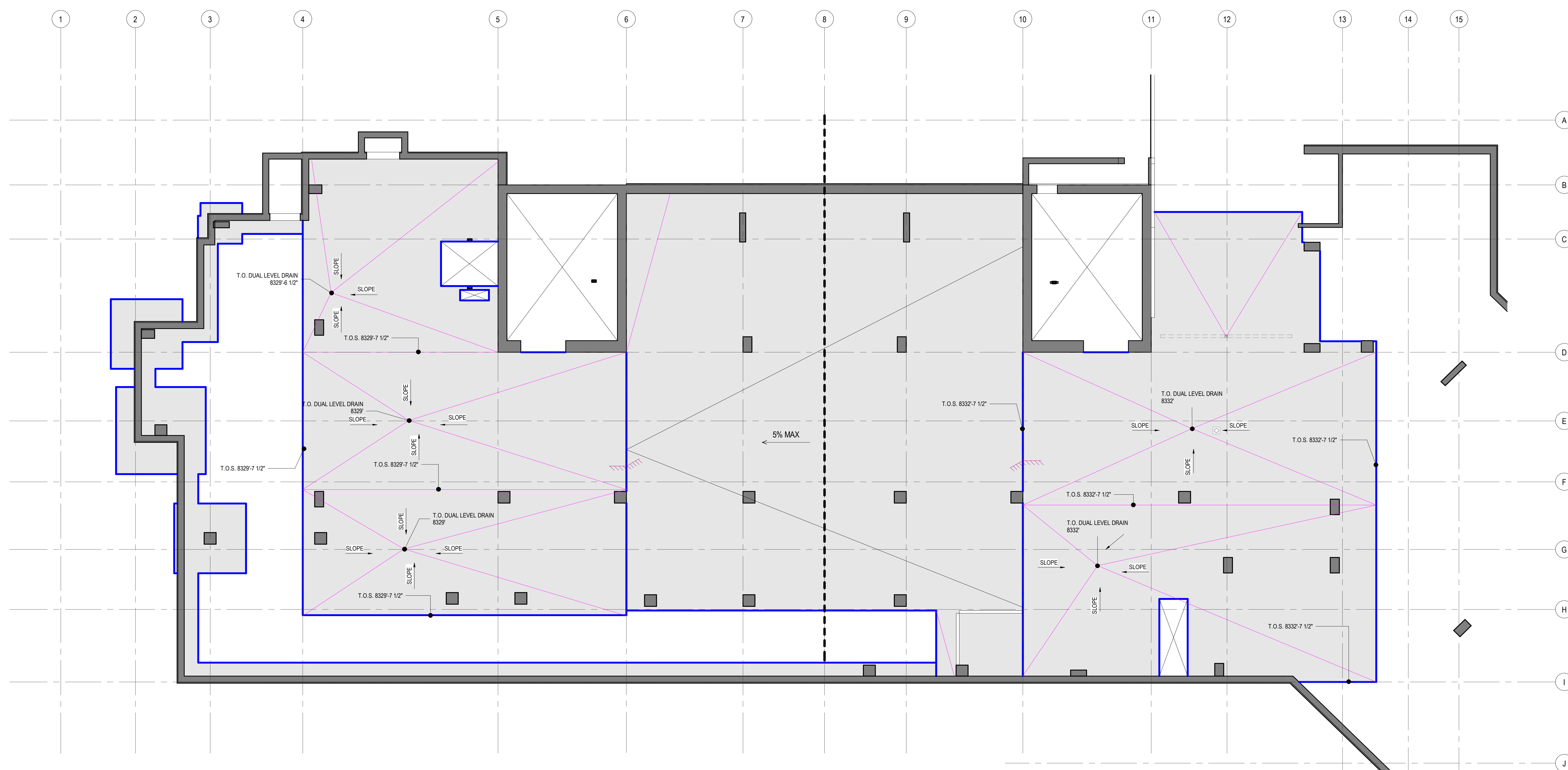
1 CONCRETE PLAN - TOWER A - LEVEL P2 SPLIT SLAB SCALE: 1/8" = 1'-0"
