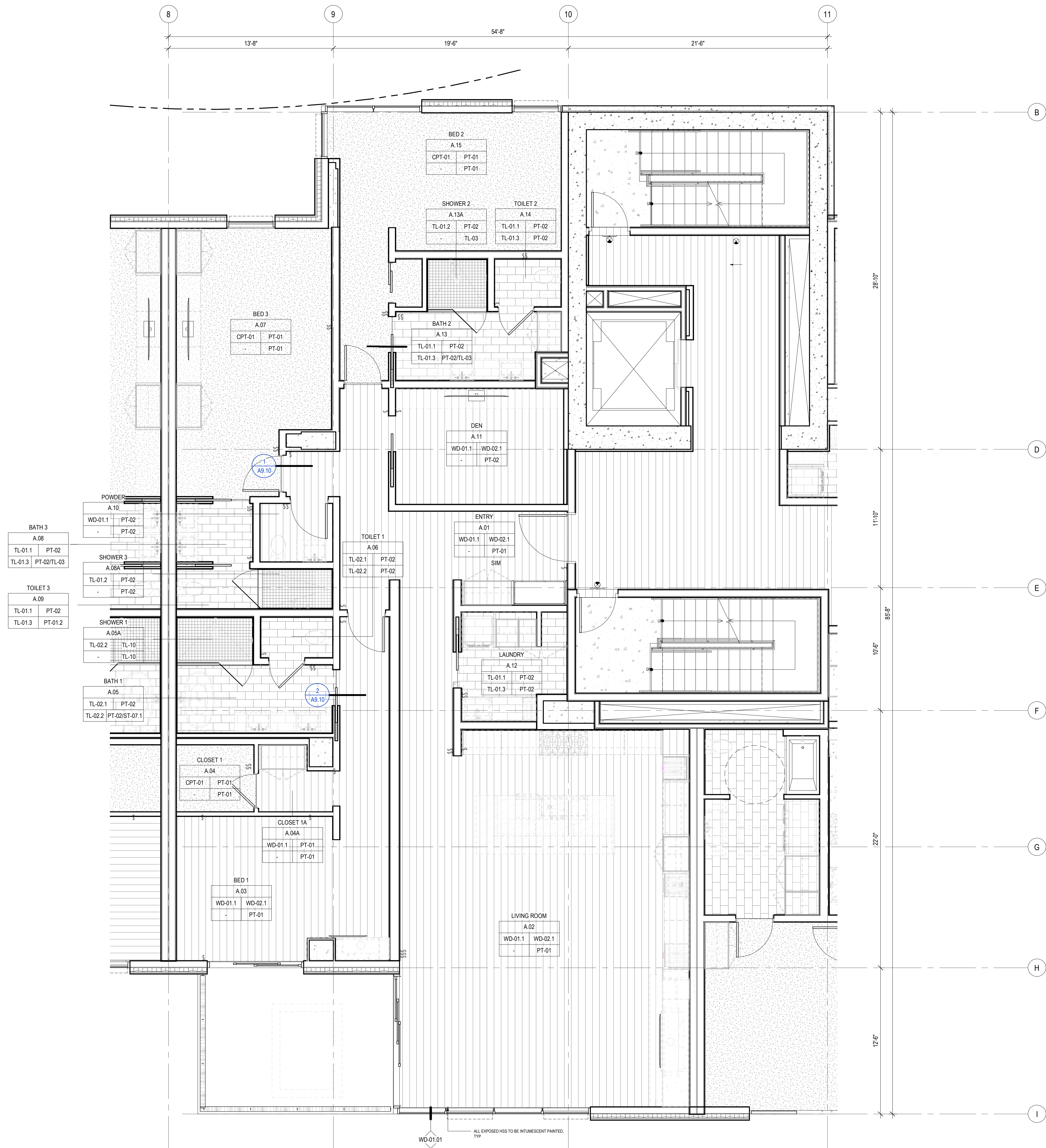
1 FINISH PLAN - TOWER A/B - UNIT A SCALE: 1/4" = 1'-0"
