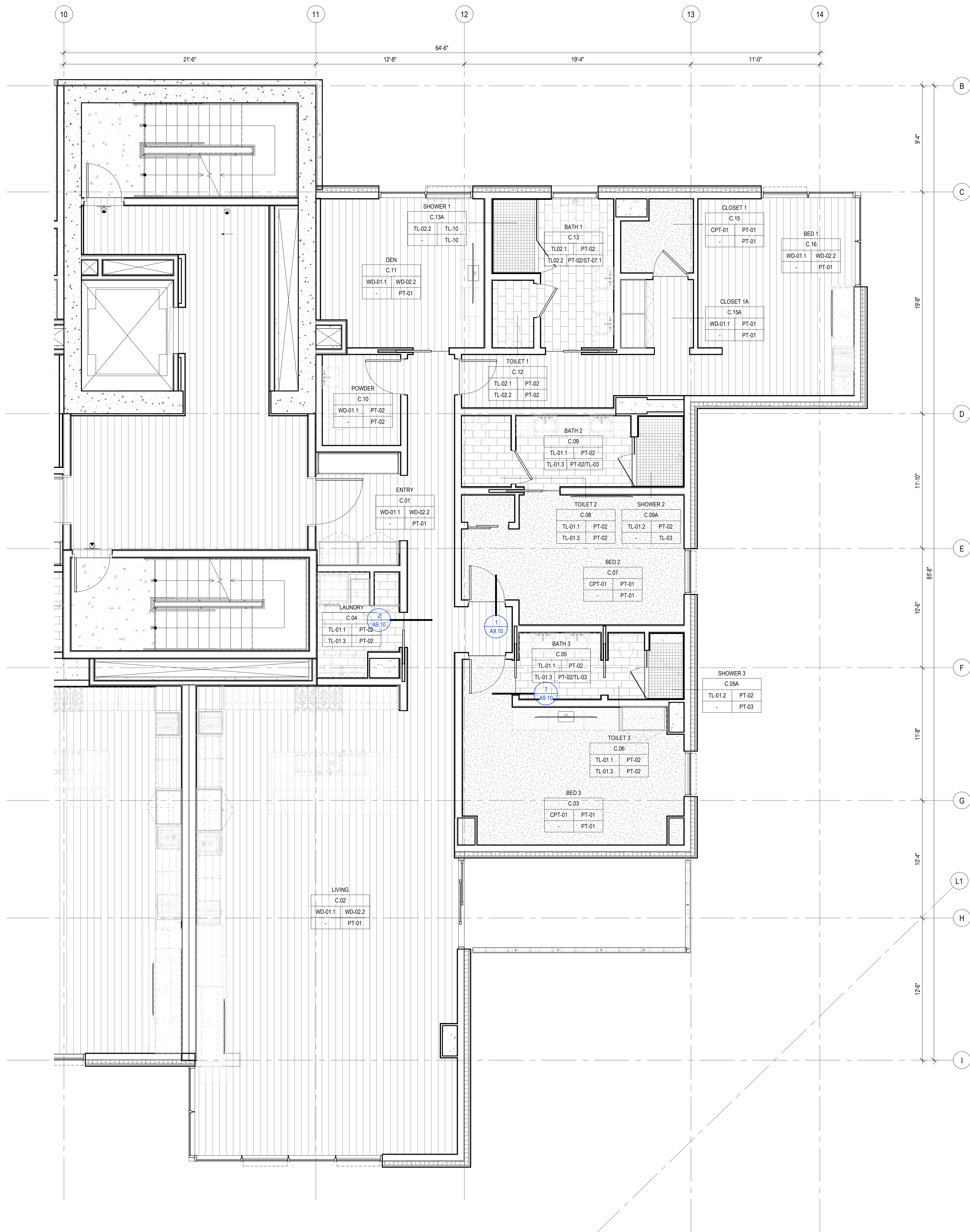
1 FINISH PLAN - TOWER A/B - UNIT C SCALE: 1/4" = 1'-0"
