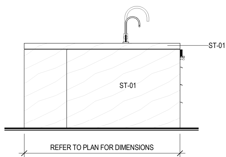
9 UNIT D - KITCHEN ISLAND - D SCALE: 1/2" = 1'-0"
