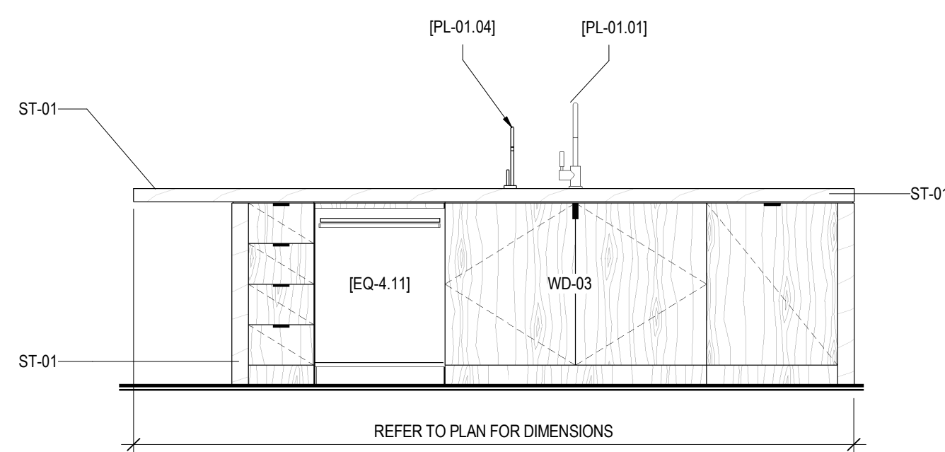
8 UNIT D - KITCHEN ISLAND - C SCALE: 1/2" = 1'-0"
