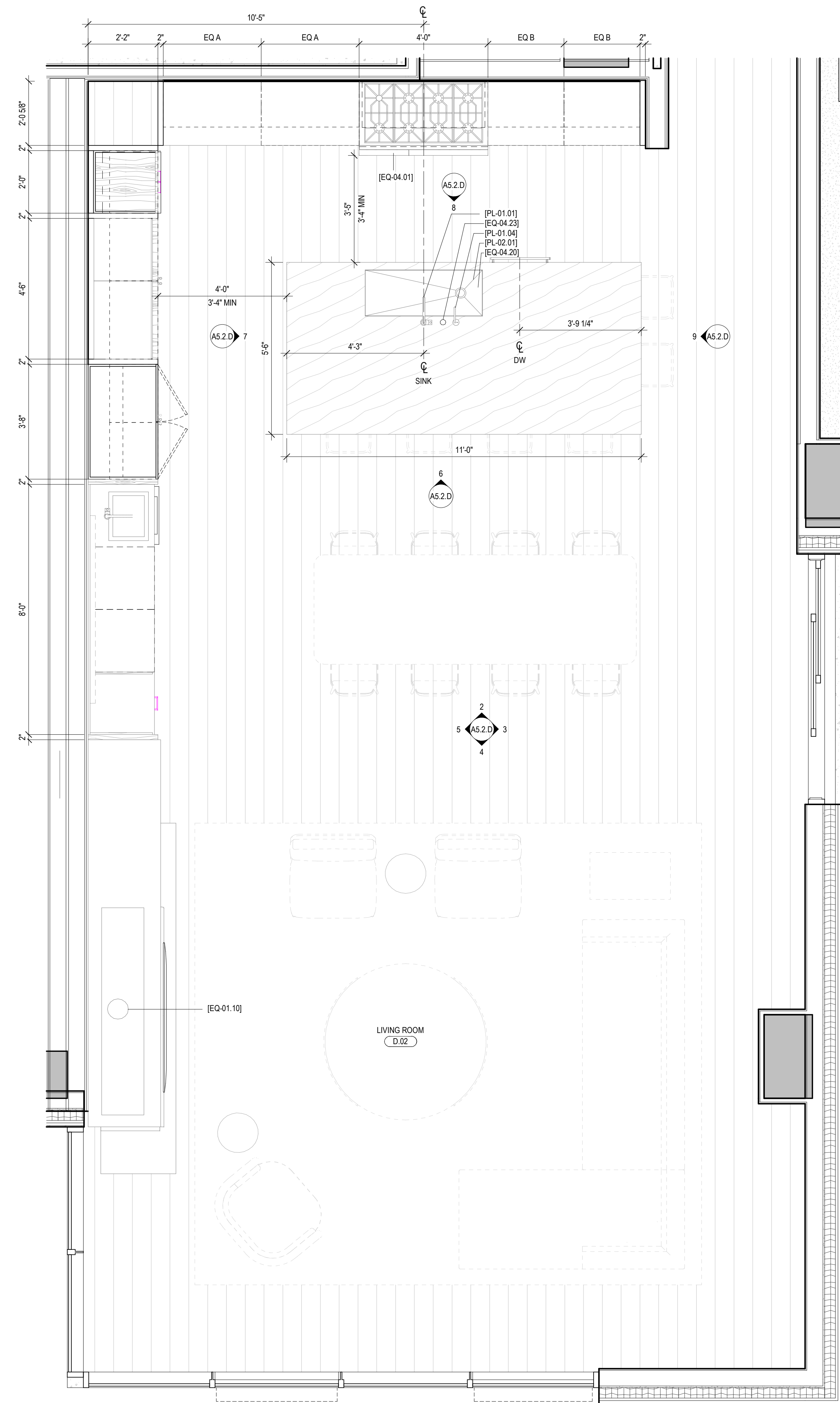
1 UNIT D - ENLARGED KITCHEN/LIVING SCALE: 1/2" = 1'-0"
