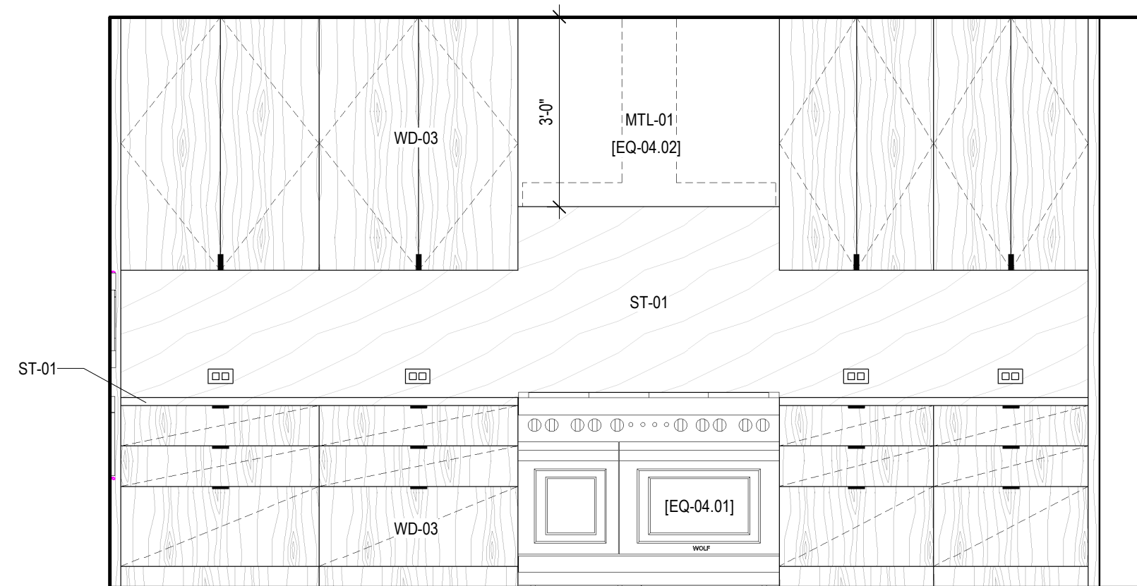
2 UNIT D - KITCHEN/LIVING - A SCALE: 1/2" = 1'-0"
