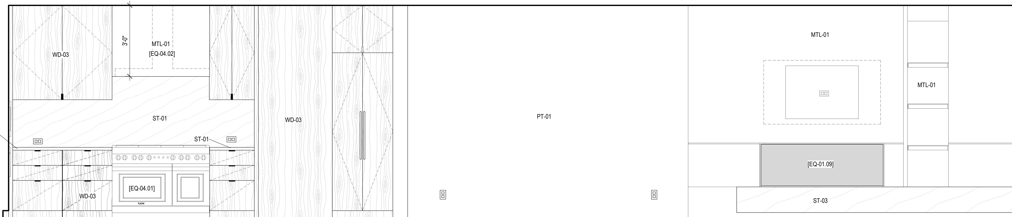
6 INTERIOR ELEVATION - UNIT G - KITCHEN/LIVING - A SCALE: 1/2" = 1'-0"
