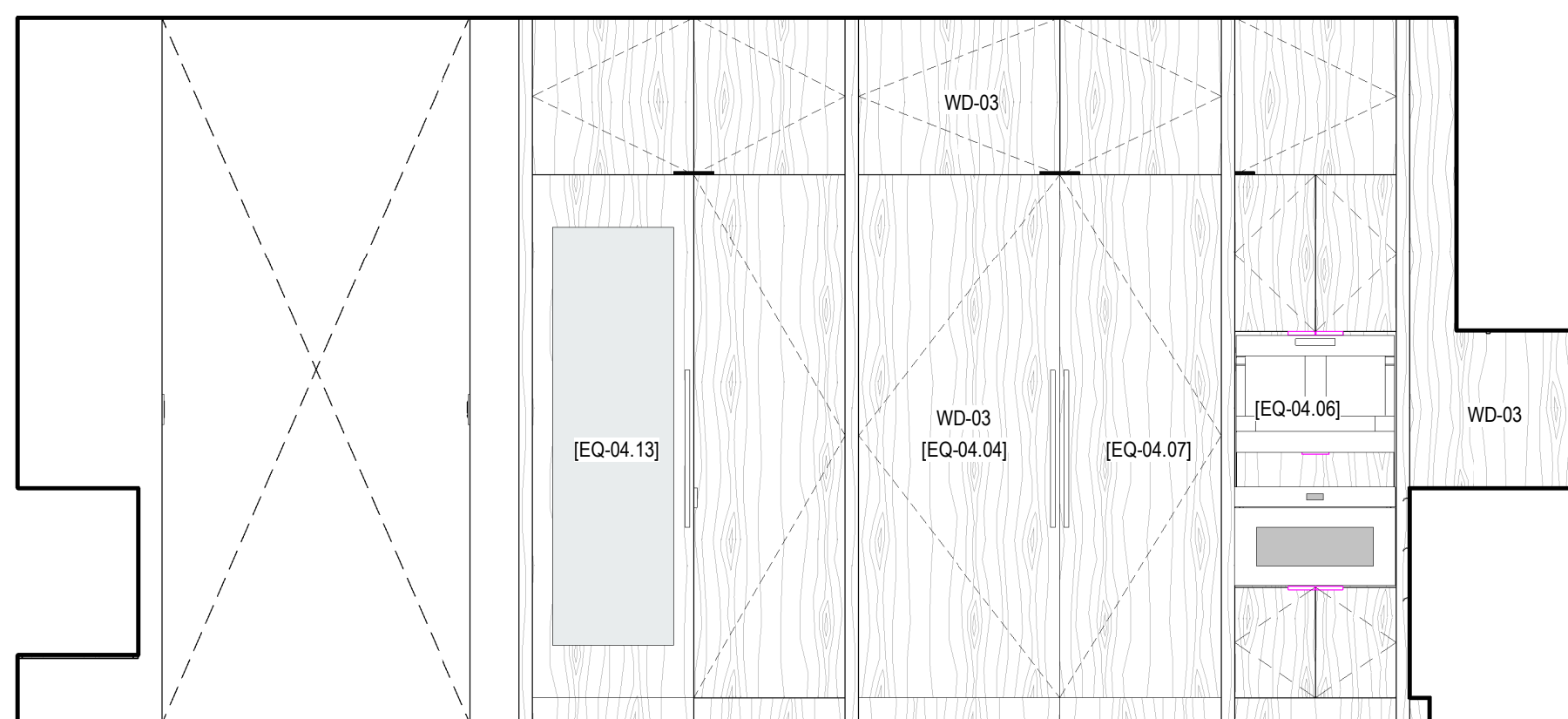
7 INTERIOR ELEVATION - UNIT G - KITCHEN/LIVING - D SCALE: 1/2" = 1'-0"
