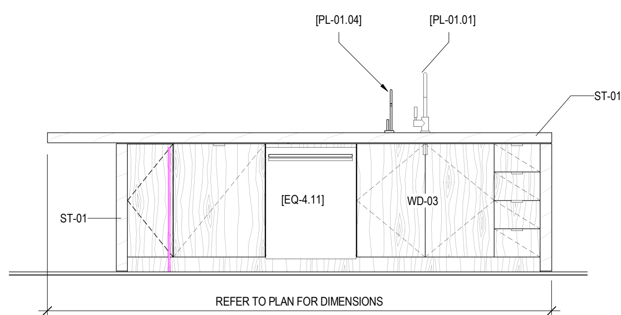
4 UNIT G - KITCHEN ISLAND - C SCALE: 1/2" = 1'-0"
