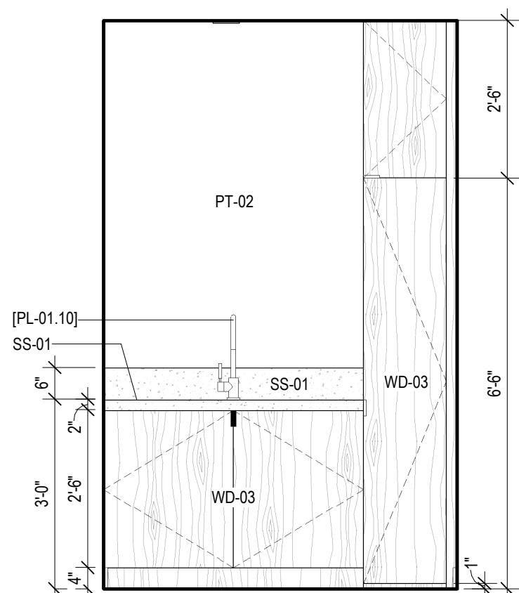
5 UNIT J - LAUNDRY - D SCALE: 1/2" = 1'-0"
