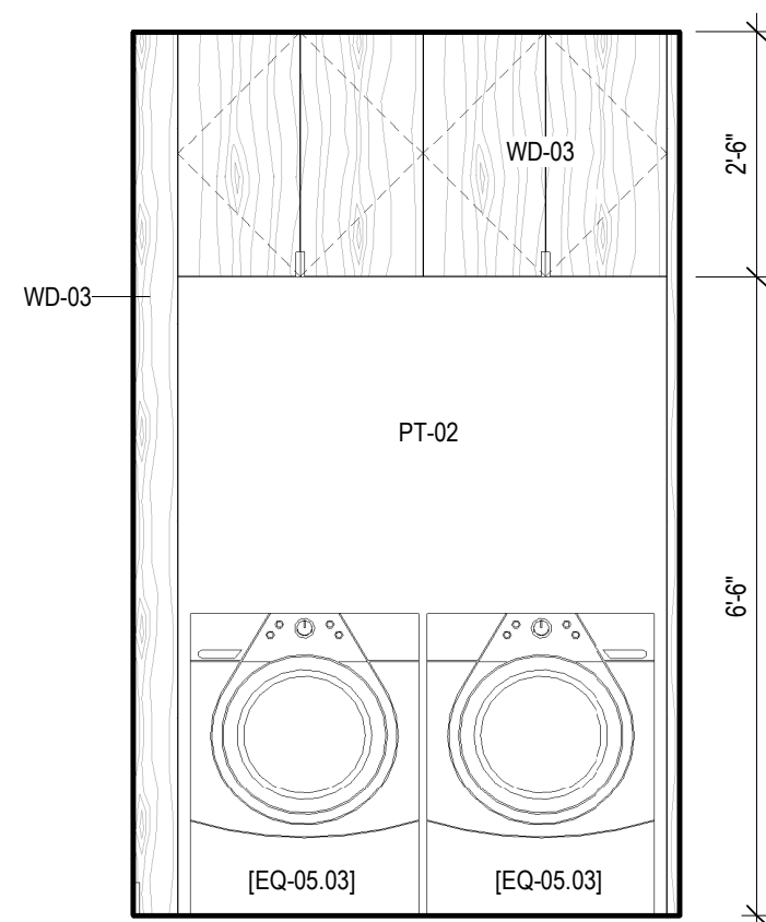
3 UNIT J - LAUNDRY - B SCALE: 1/2" = 1'-0"
