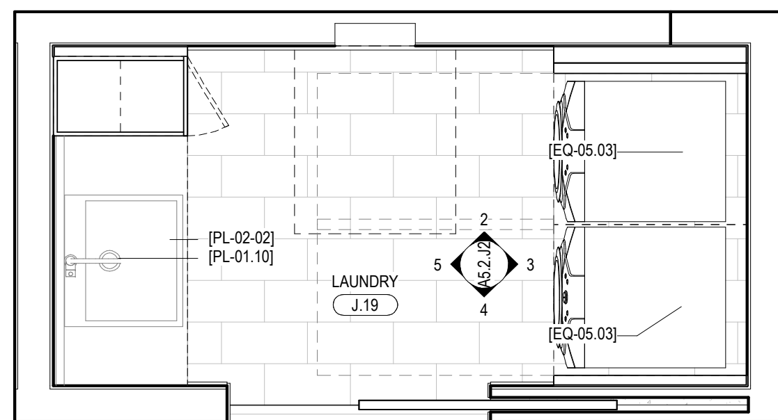
1 UNIT J - ENLARGED LAUNDRY SCALE: 1/2" = 1'-0"
