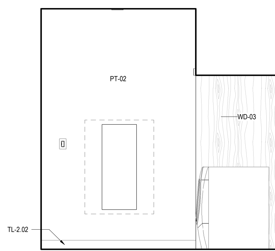
2 UNIT J - LAUNDRY - A SCALE: 1/2" = 1'-0"
