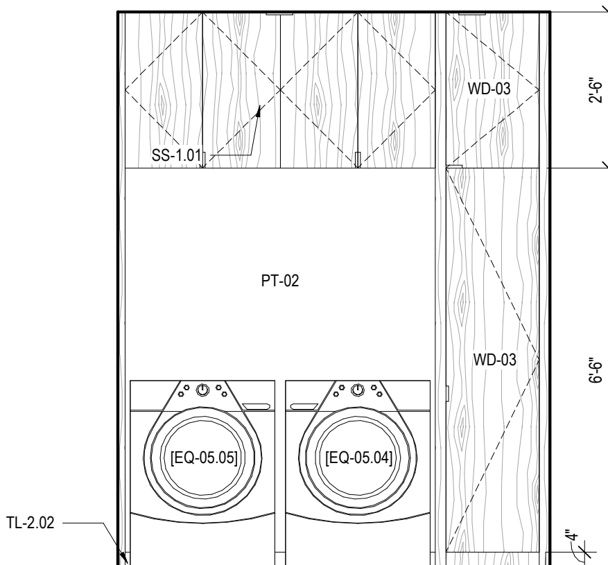
5 UNIT K - LAUNDRY - D SCALE: 1/2" = 1'-0"
