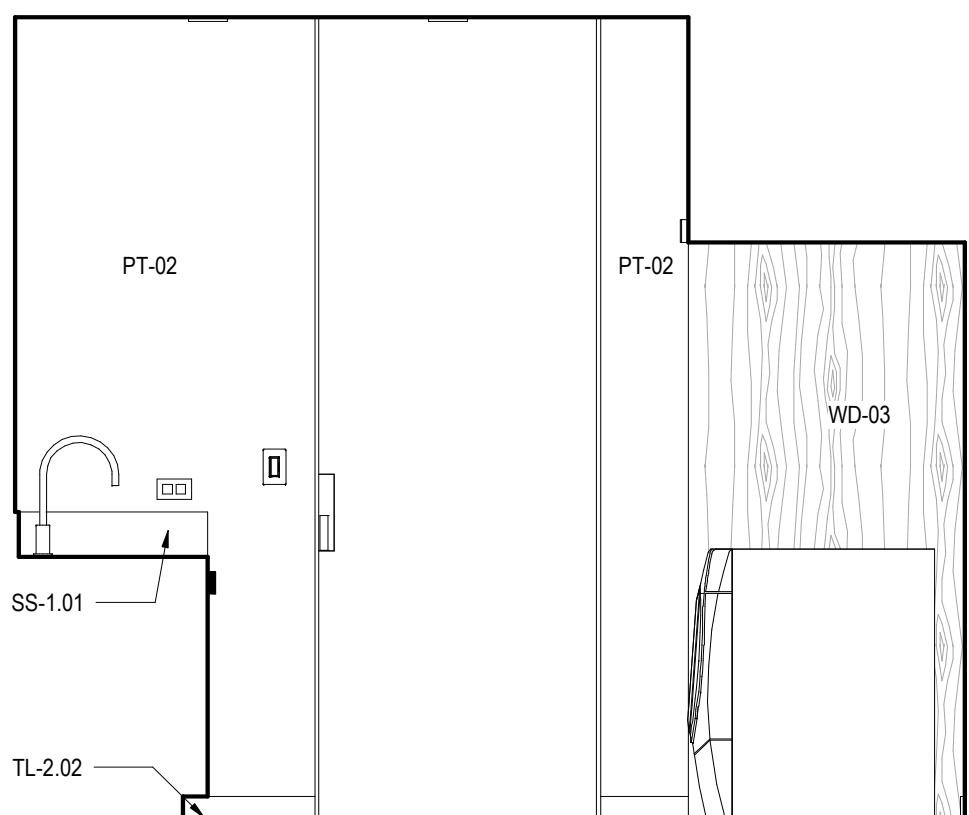
4 UNIT K - LAUNDRY - C SCALE: 1/2" = 1'-0"
