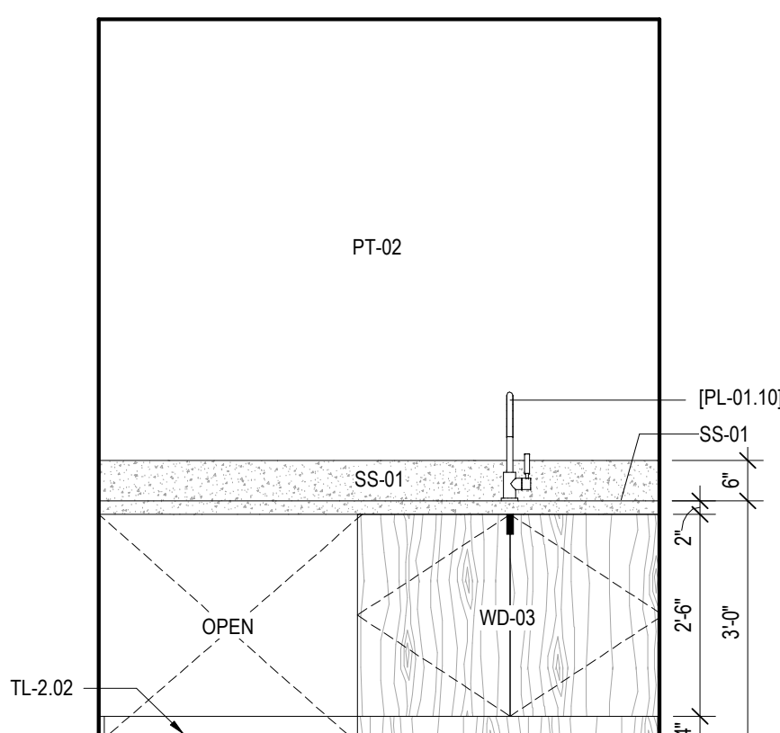
3 UNIT K - LAUNDRY - B SCALE: 1/2" = 1'-0"
