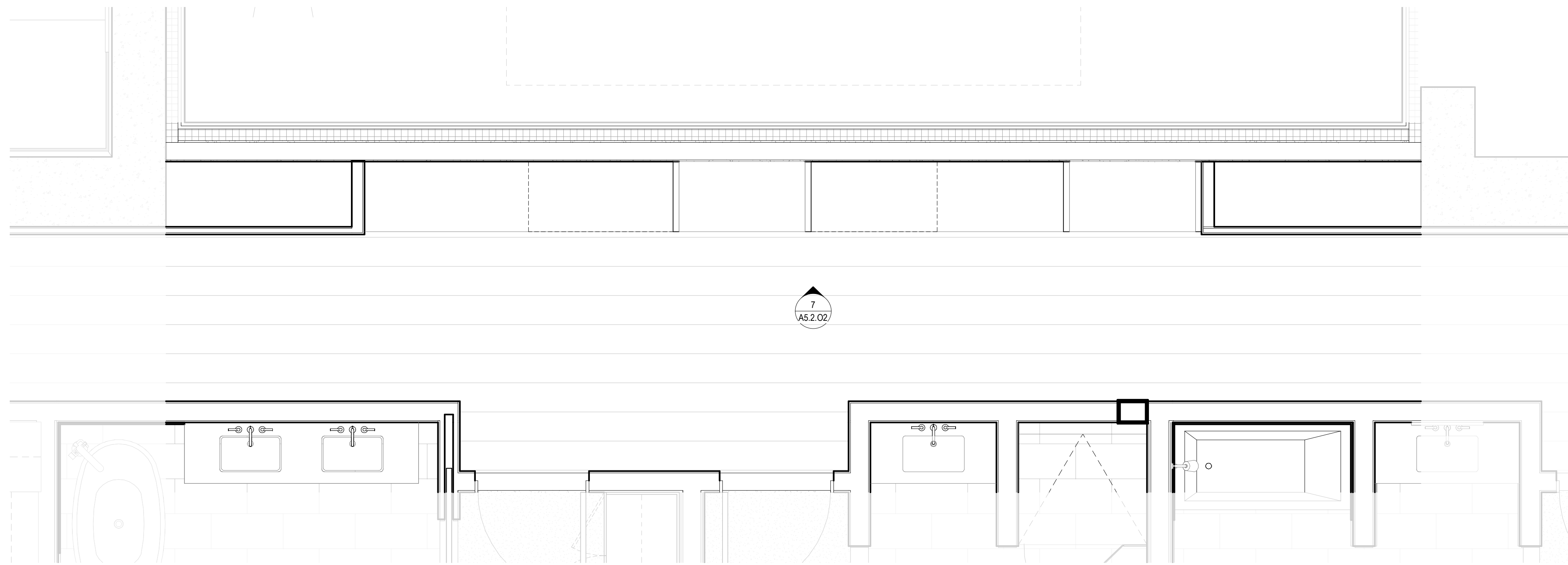
6 ENLARGED PLAN - UNIT O - CORRIDOR SCALE: 1/2" = 1'-0"
