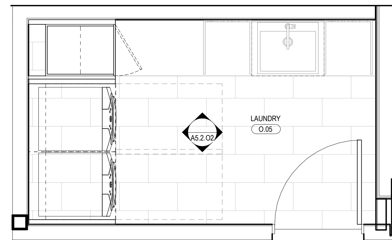
1 ENLARGED PLAN - UNIT O - LAUNDRY SCALE: 1/2" = 1'-0"
