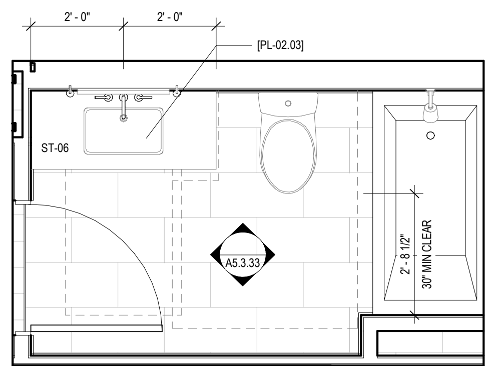
11 ENLARGED PLAN - ANSI OPTION A - LAYOUT 4 SCALE: 1/2" = 1'-0"
