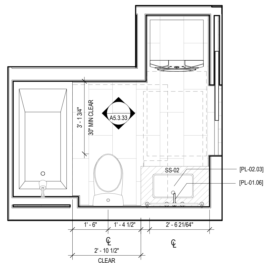
6 ENLARGED PLAN - ANSI OPTION A - LAYOUT 3 SCALE: 1/2" = 1'-0"
