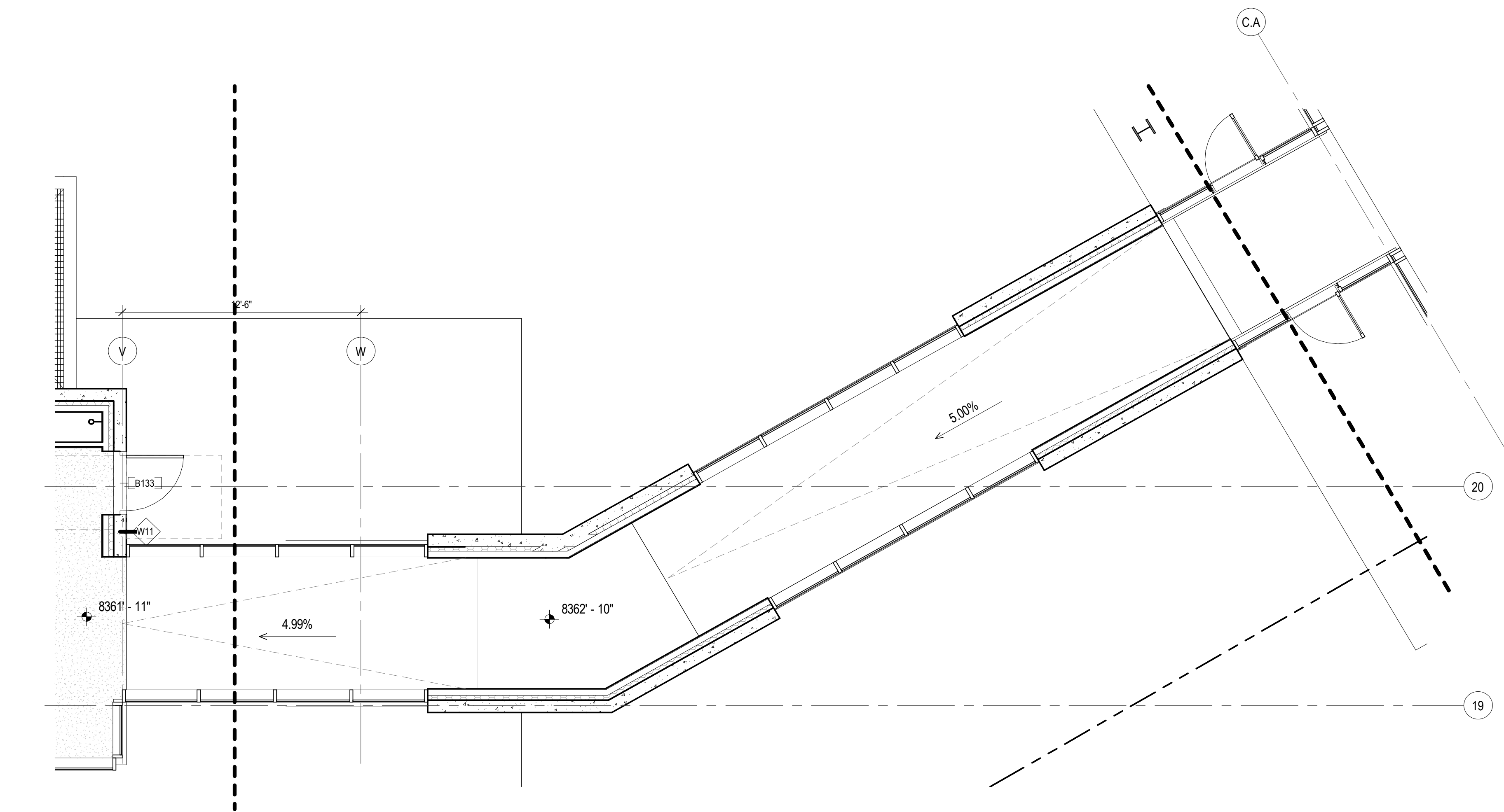
2 ENLARGED PLAN - SLOPED FLOOR - R1 SCALE: 1/4" = 1'-0"
