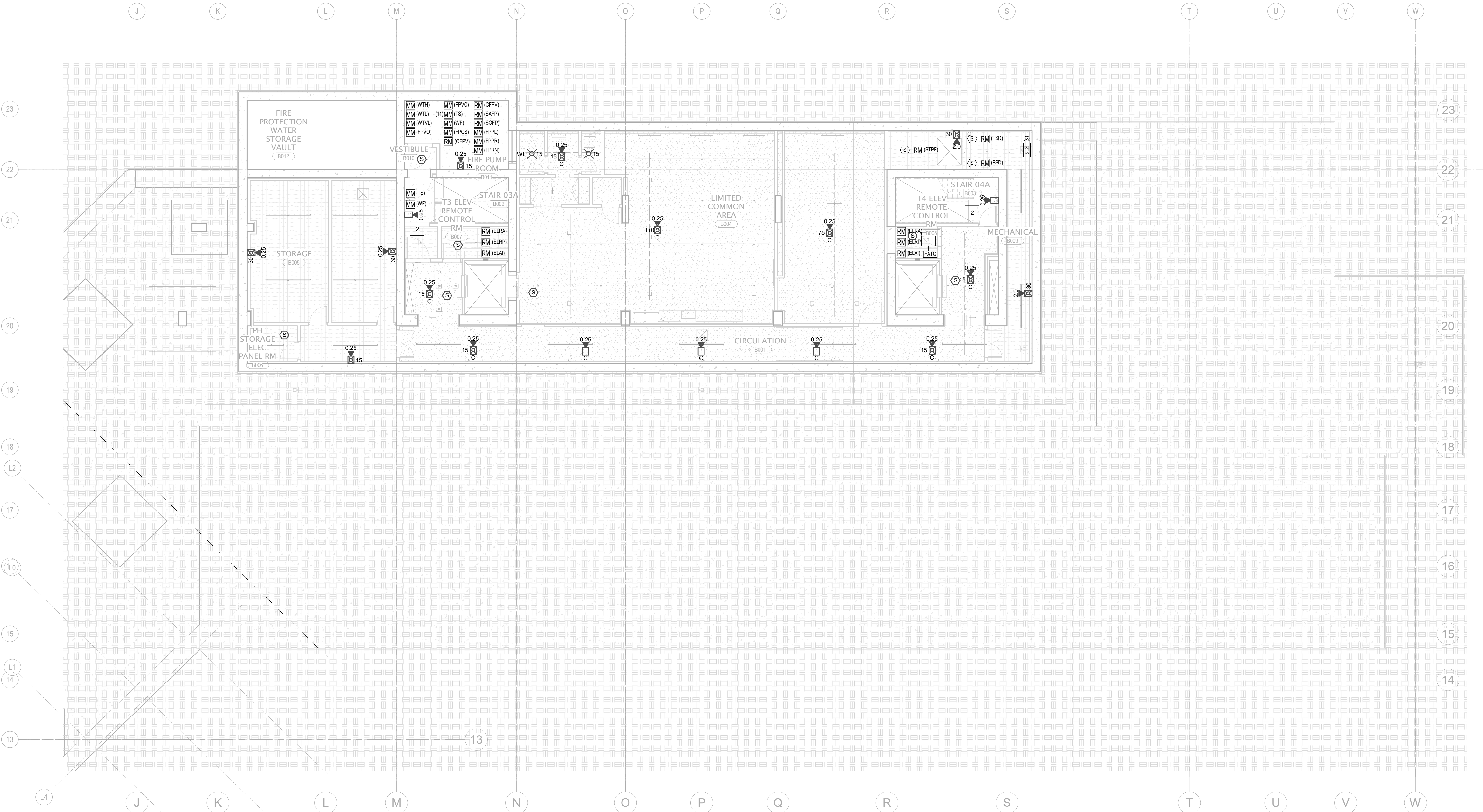
1 TOWER B - LEVEL B1 - FA 1/8" = 1'-0"
