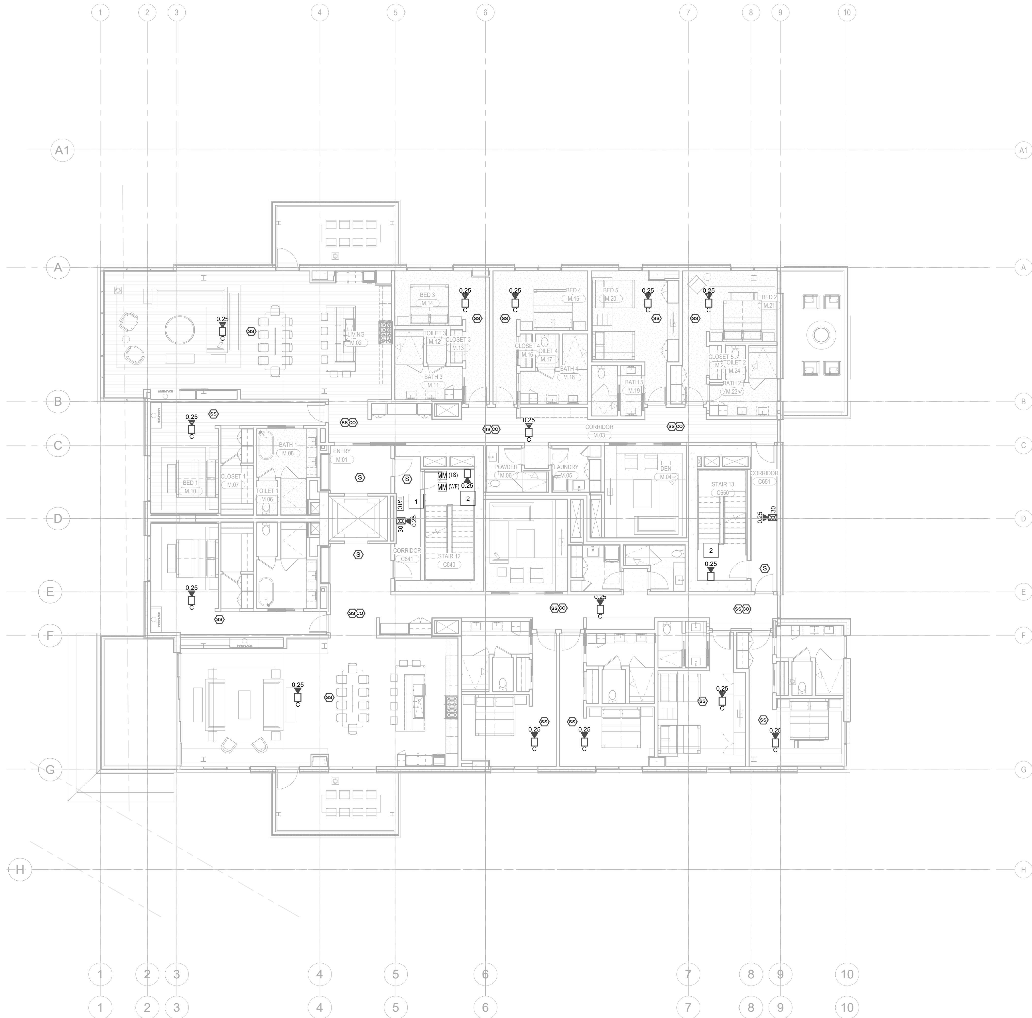
1 LEVEL 6 - FA 1/8" = 1'-0"
