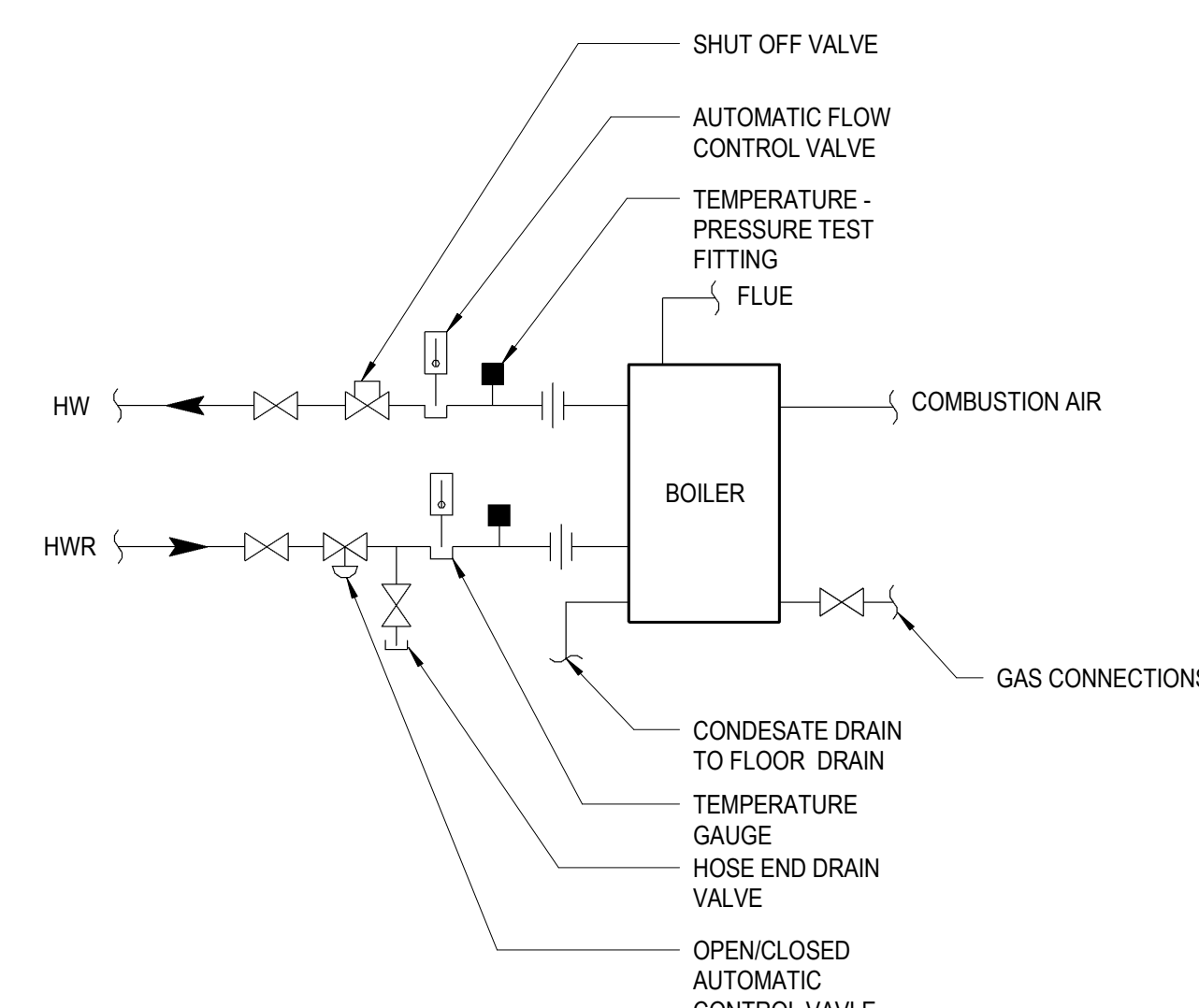
3 BOILER CONNECTION DETAIL
