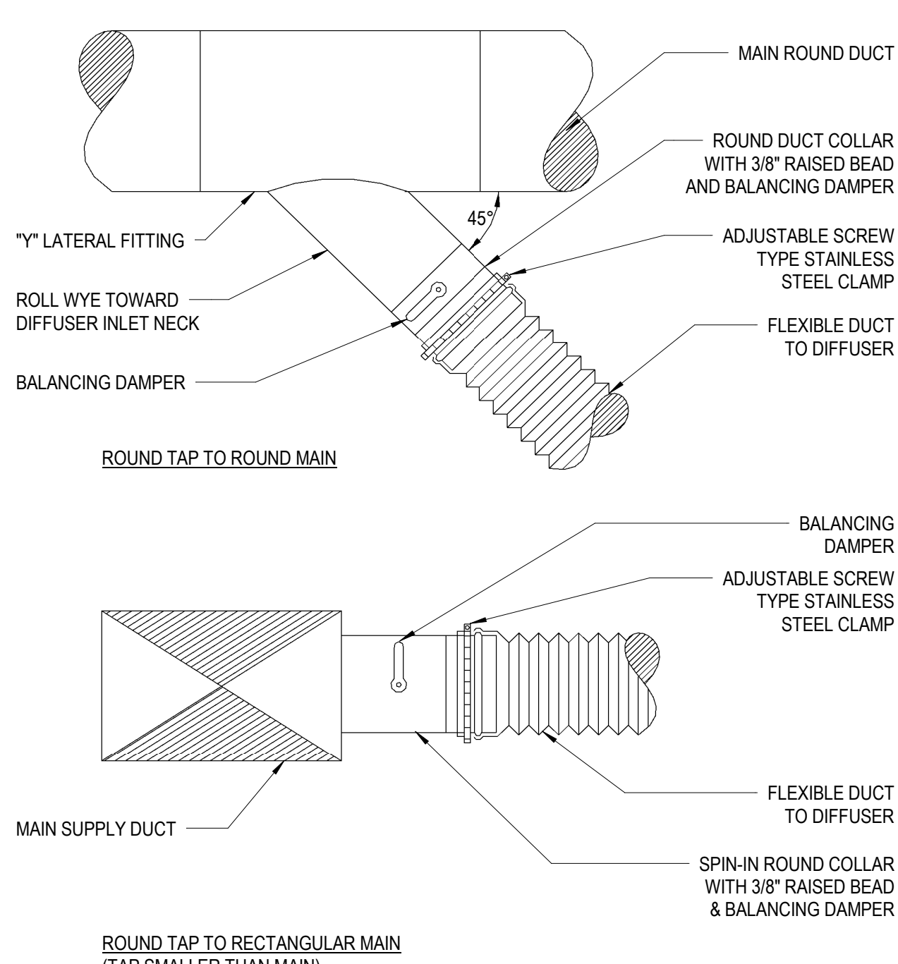
6 LOW PRESSURE BRANCH DUCT CONNECTIONS SCALE: NTS
