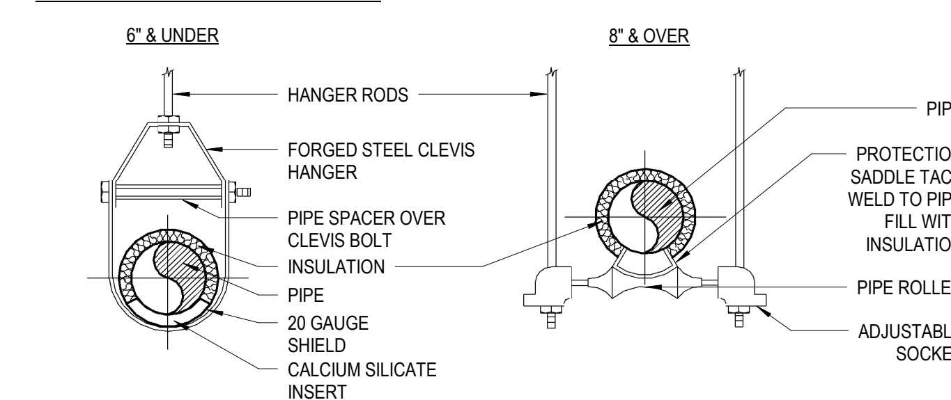
4 HOT AND CHILLED WATER PIPE HANGER SINGLE PIPE SCALE: NTS
