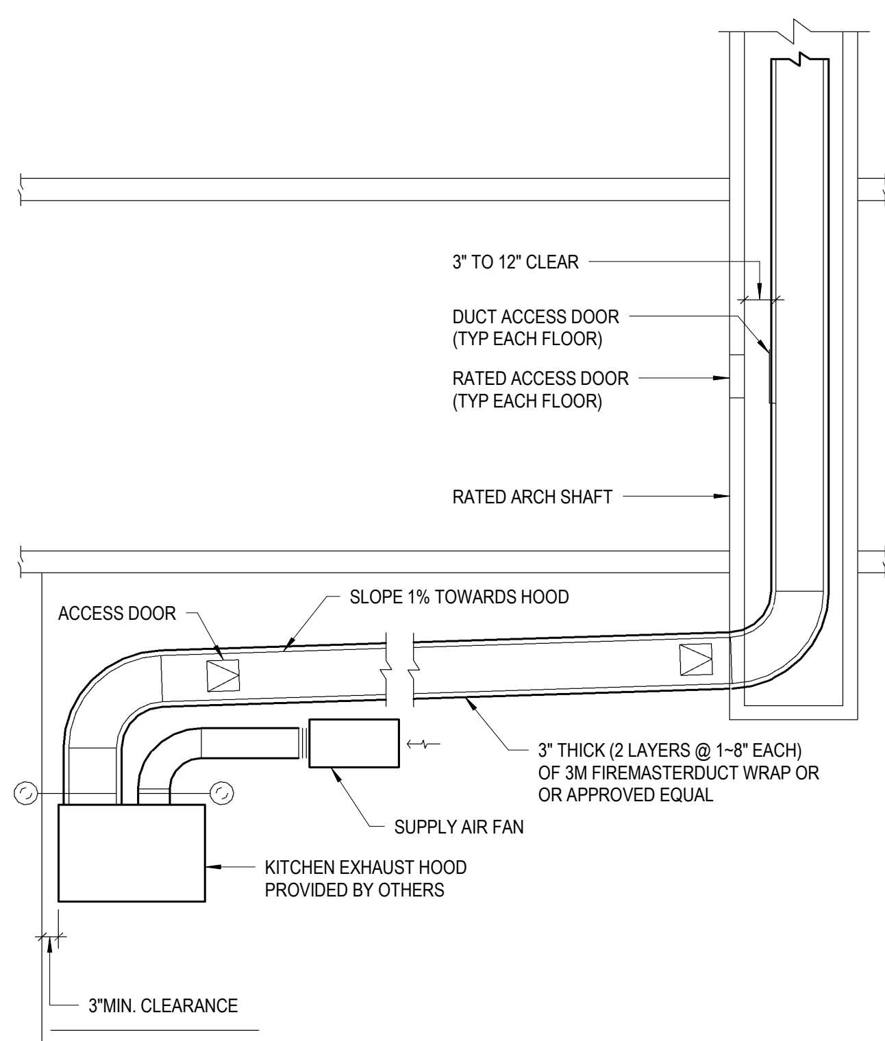
8 KITCHEN HOOD EXHAUST RISER DETAIL SCALE: NTS
