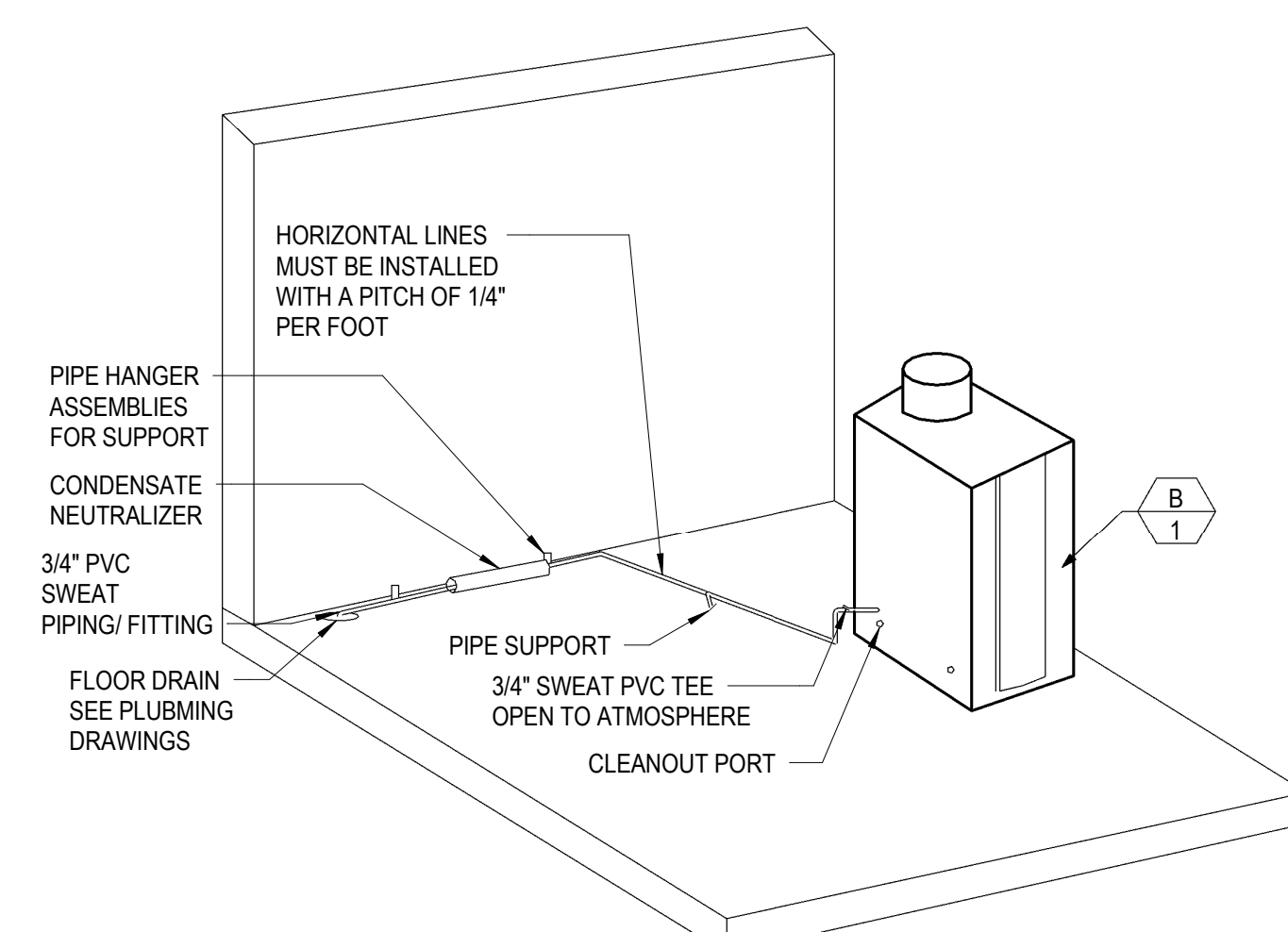
5 BOILER CONDENSATE DRAIN DETAIL SCALE: NTS
