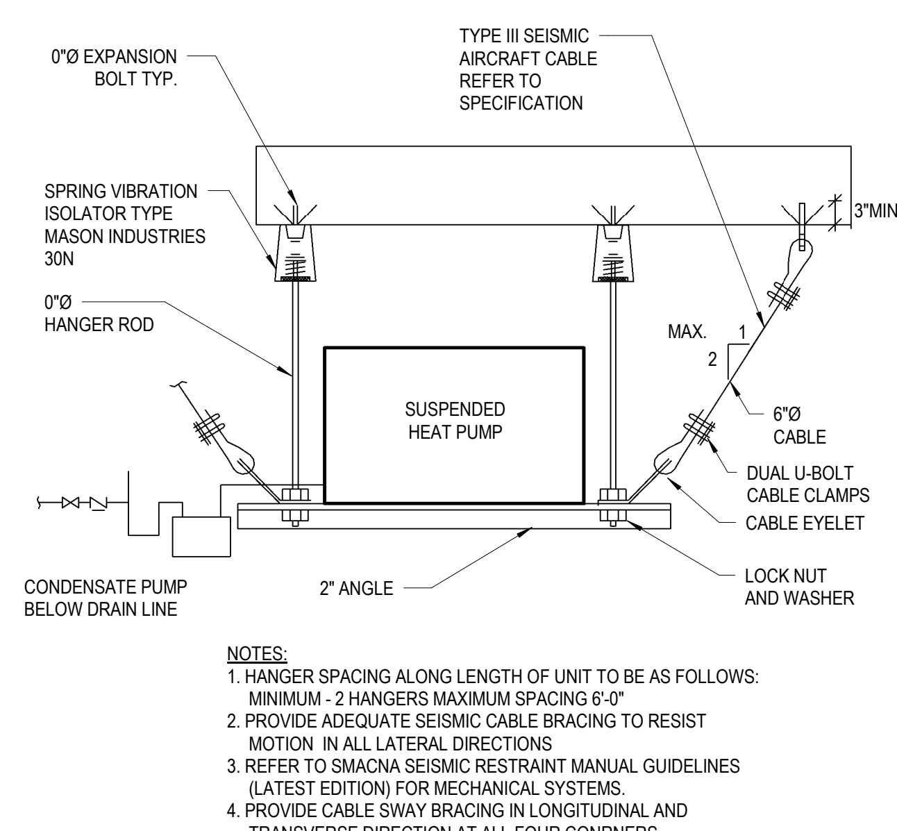
9 SUSPENDED EQUIPMENT WITH SEISMIC CABLES - A
