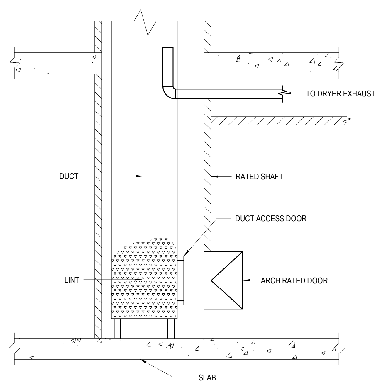
1 DRYER EXHAUST LINT TRAP SCALE: NTS
