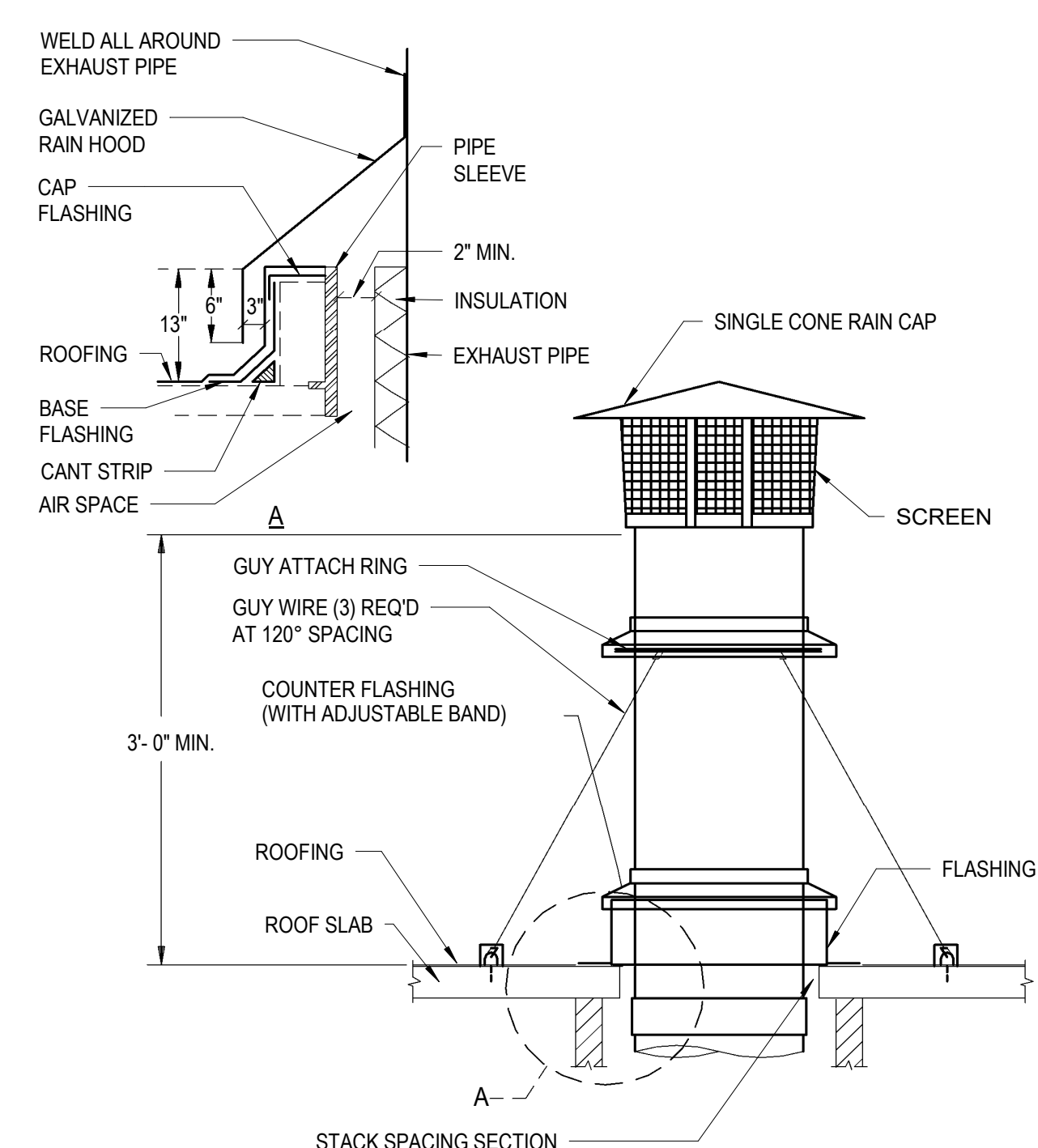
2 CONDENSING BOILER FLUE THRU ROOF SCALE: NTS
