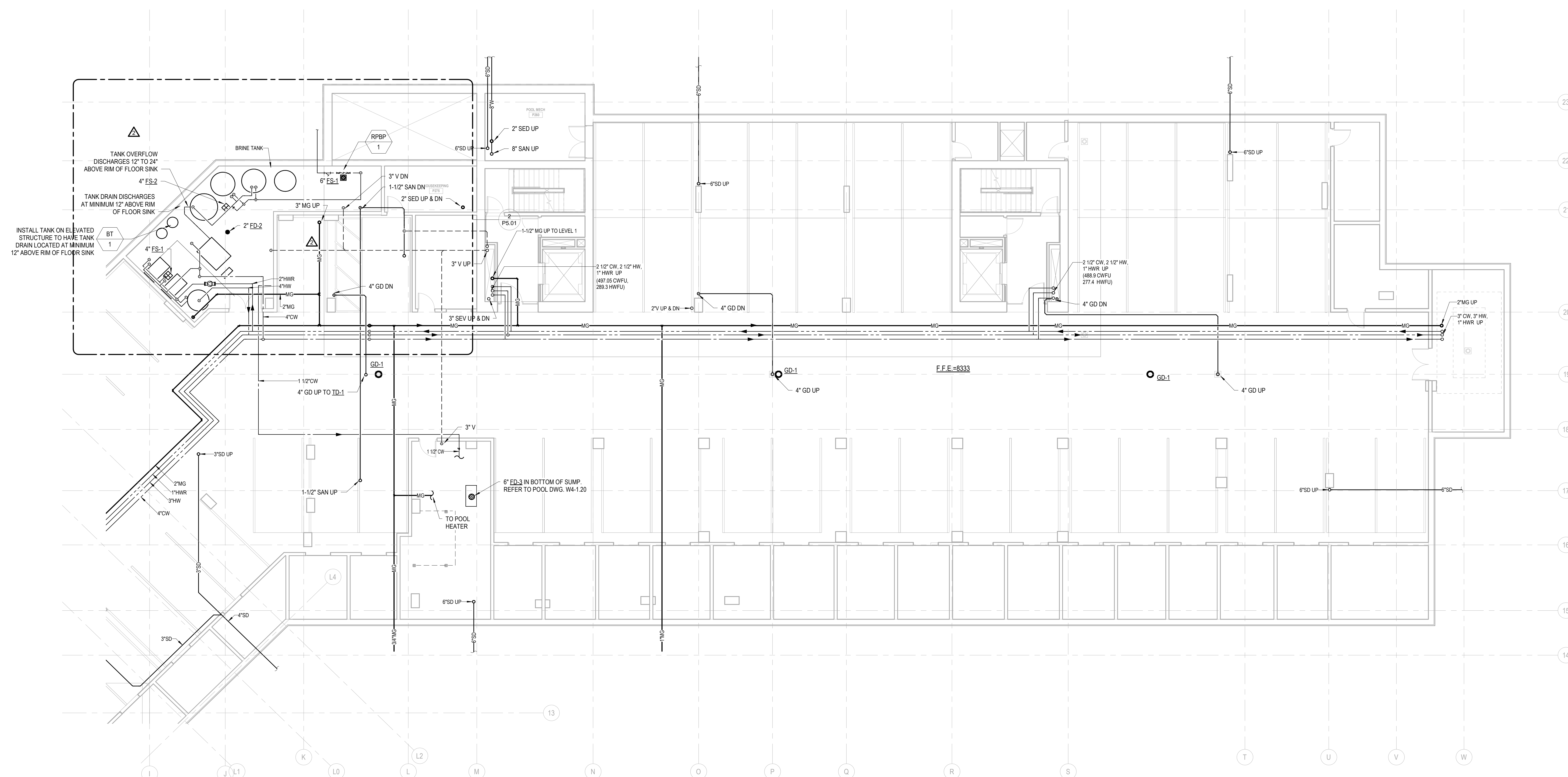
1 PLAN - TOWER B - LVL P2 SCALE: 1/8" = 1'-0"
