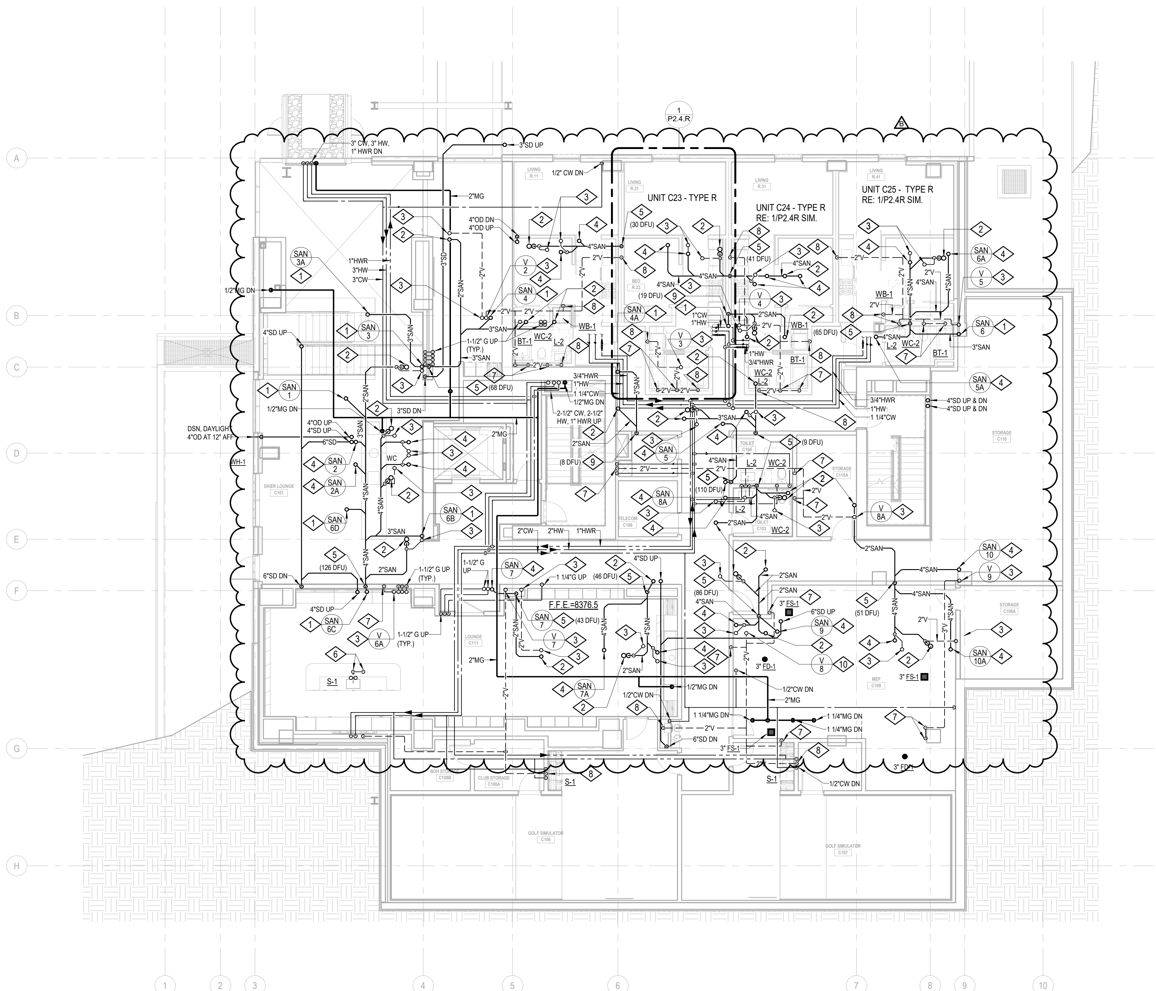
1 PLAN - TOWER C - LVL 1 SCALE: 1/8" = 1'-0"
