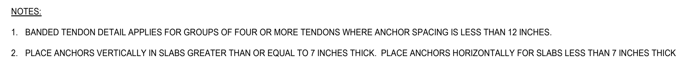
DISTRIBUTED TENDONS
