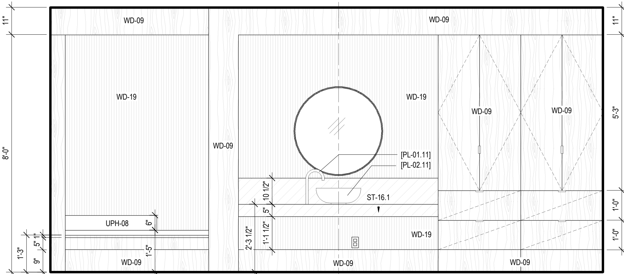
11 SPA TREATMENT DOUBLE, 187 - A SCALE: 1/2" = 1'-0"
