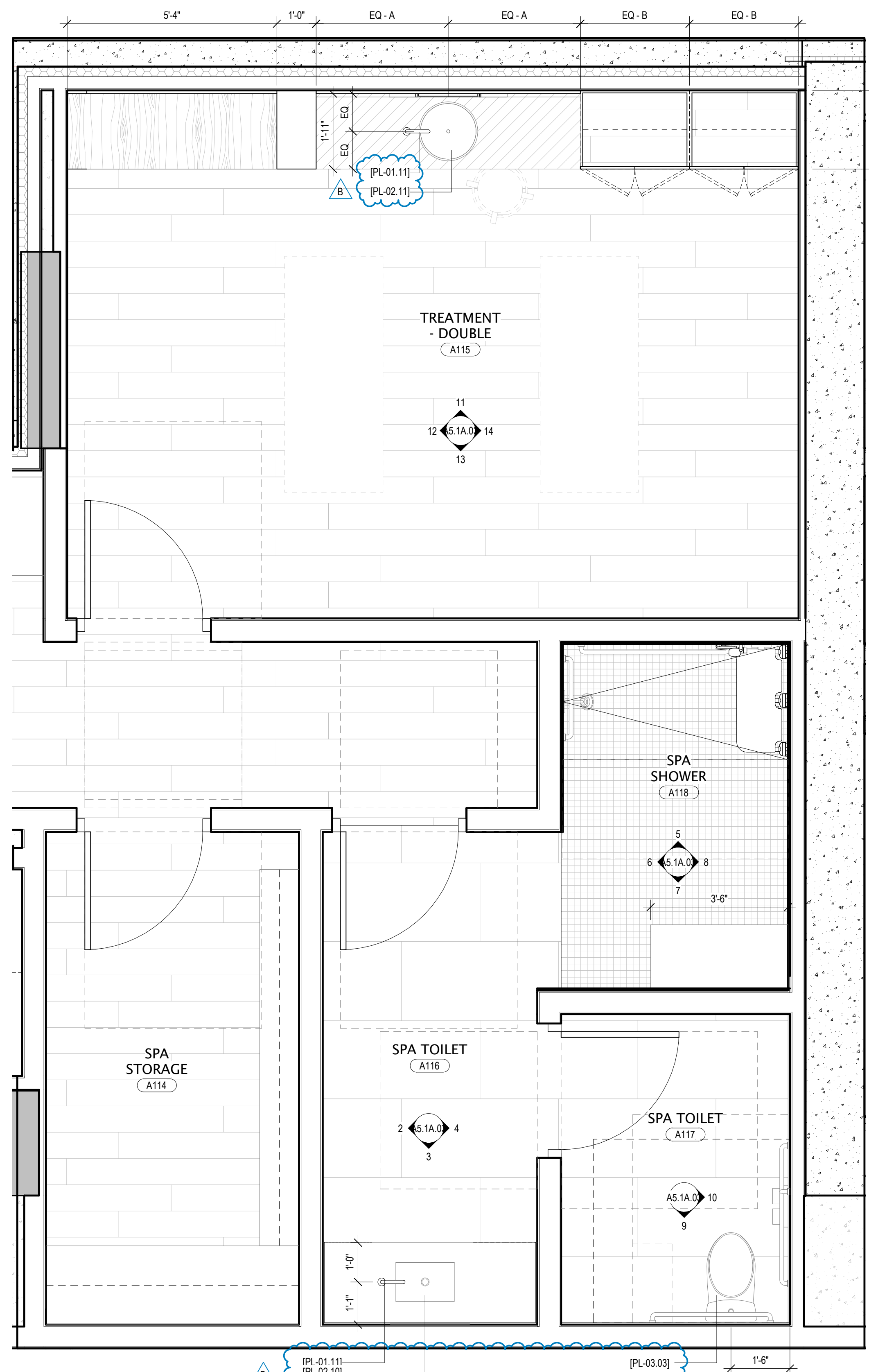
1 ENLARGED PLAN, SPA TREATMENT - DOUBLE SCALE: 1/2" = 1'-0"
