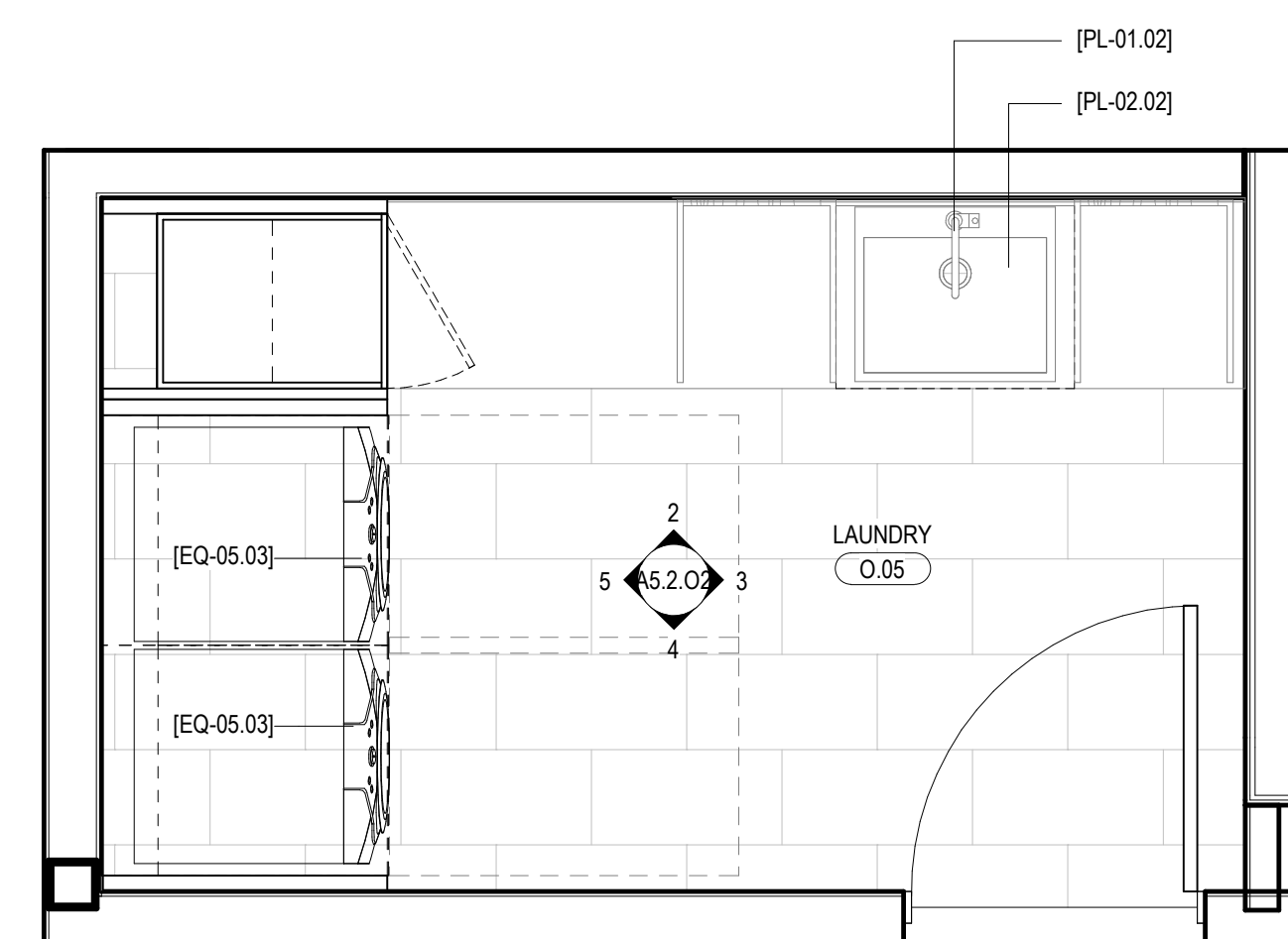
1 ENLARGED PLAN - UNIT O - LAUNDRY SCALE: 1/2" = 1'-0"
