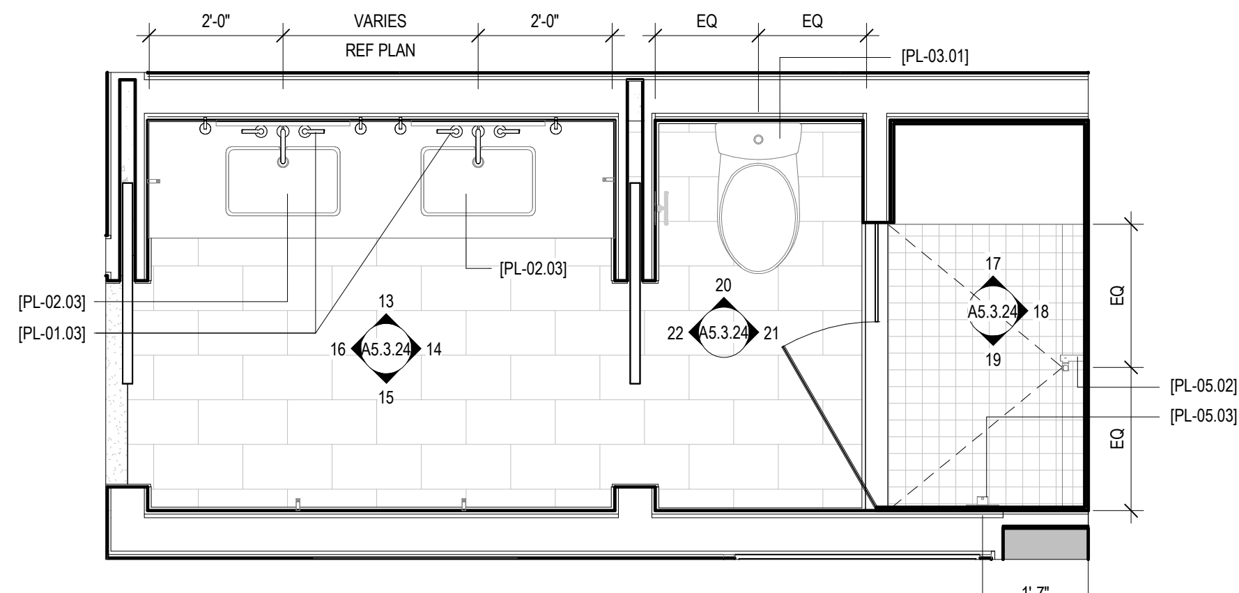
12 ENLARGED PLAN - BATH 9 SCALE: 1/2" = 1'-0"
