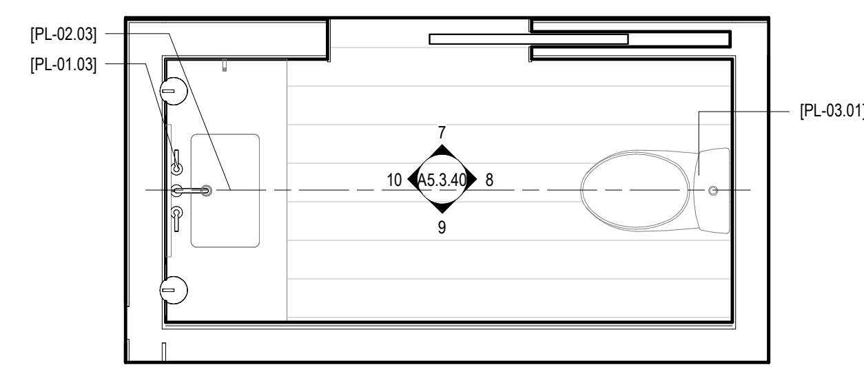
6 ENLARGED PLAN - POWDER 2 SCALE: 1/2" = 1'-0"
