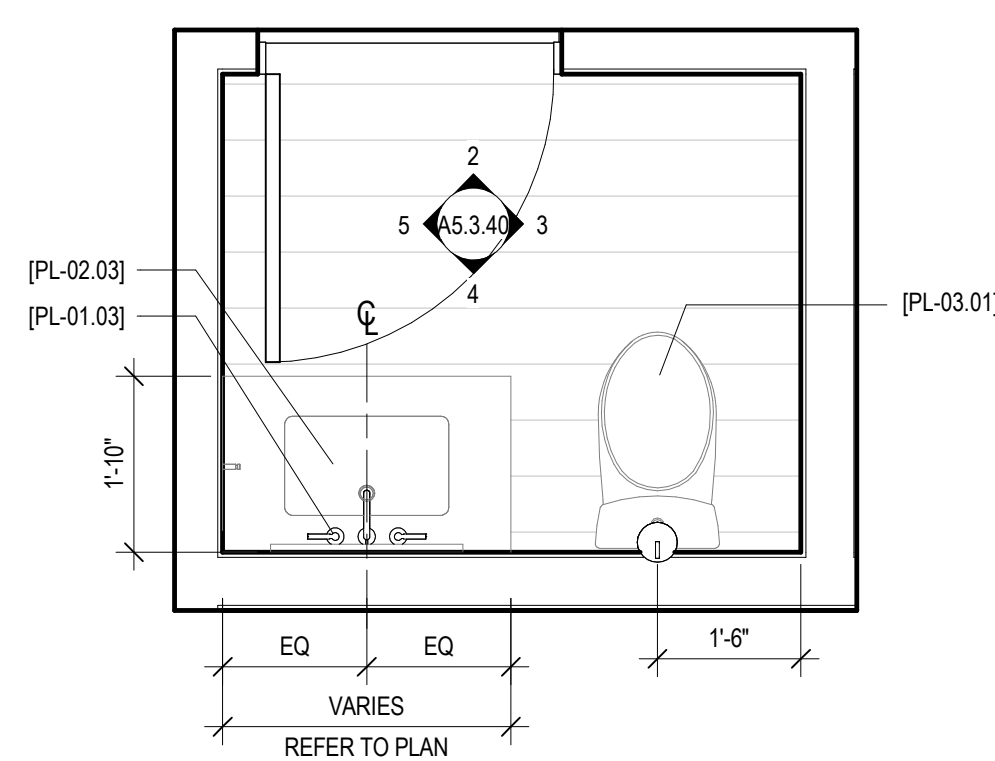
1 ENLARGED PLAN - POWDER 1 SCALE: 1/2" = 1'-0"
