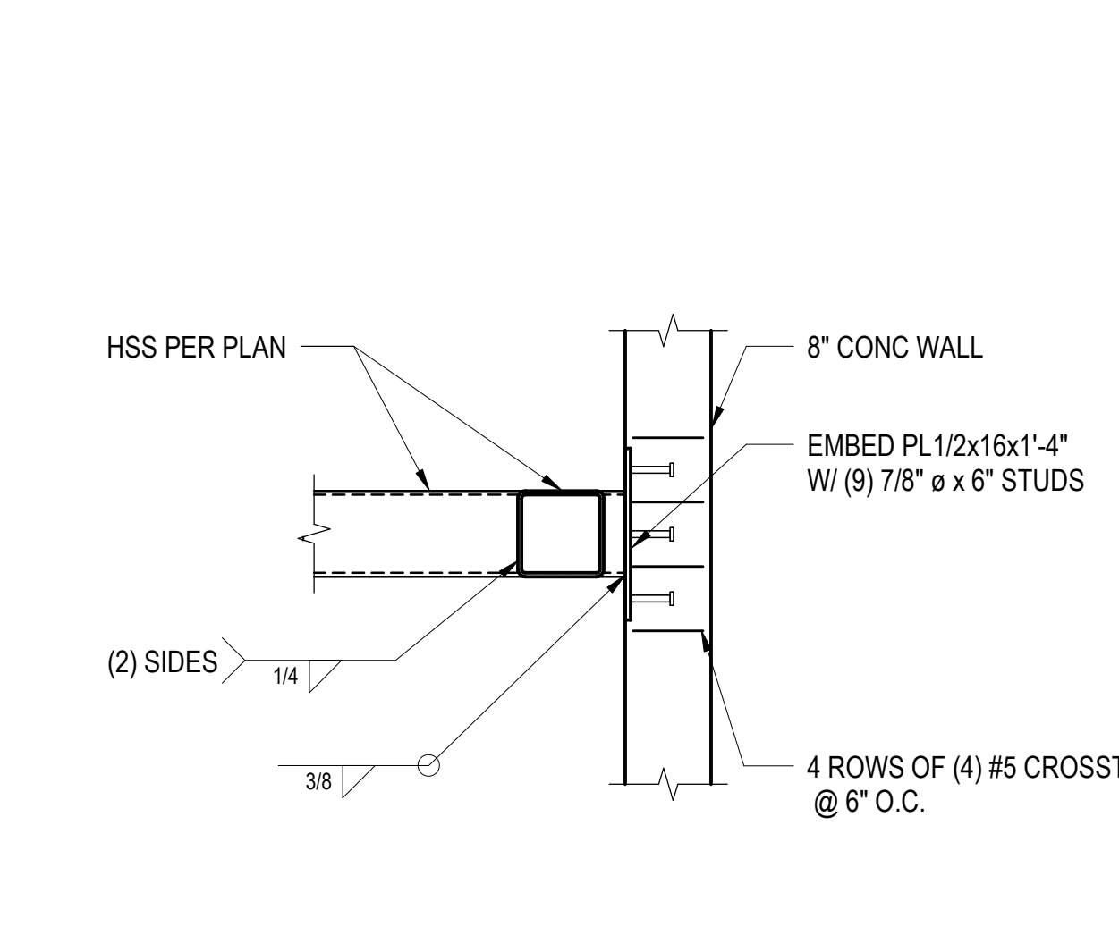
10 SECTION 3/4" = 1'-0"
