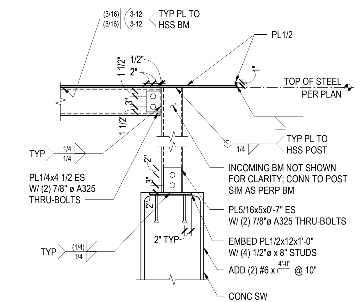
20 SECTION 3/4" = 1'-0"
