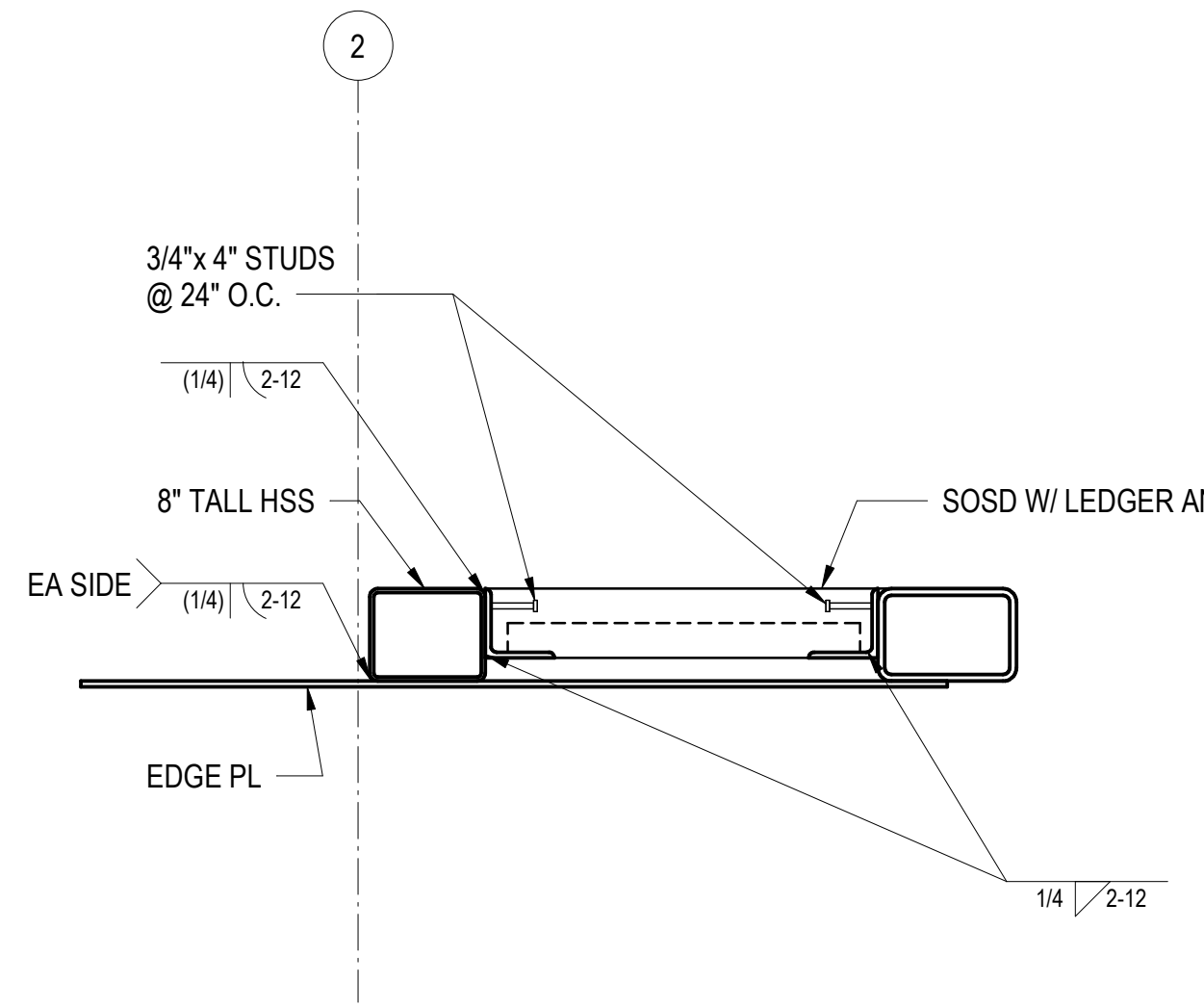
6 SECTION 3/4" = 1'-0"
