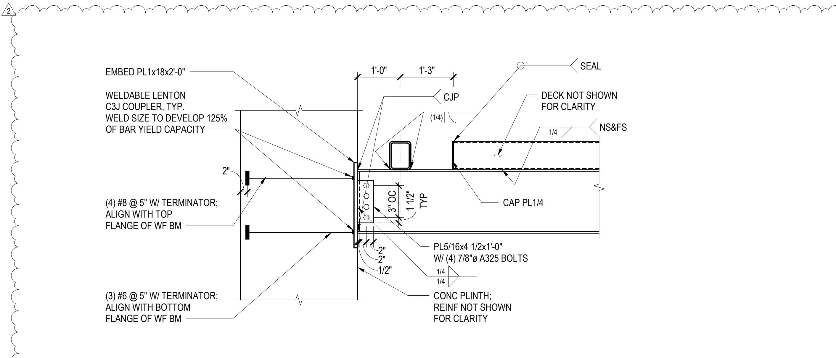
15 SECTION 3/4" = 1'-0"
