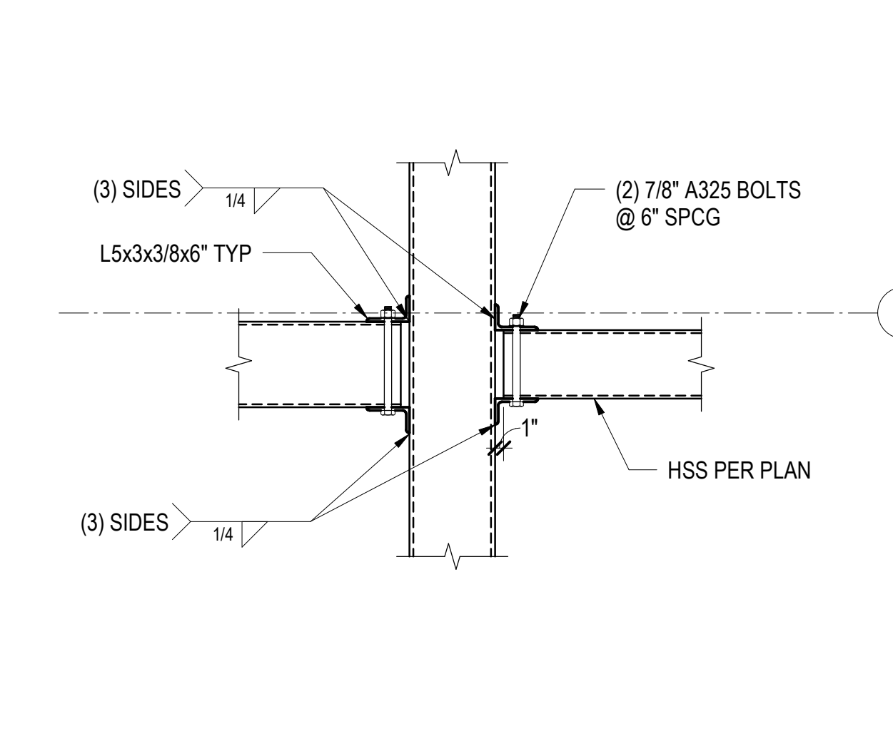
7 SECTION 3/4" = 1'-0"
