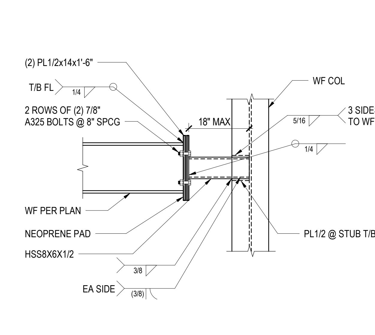
4 SECTION 3/4" = 1'-0"
