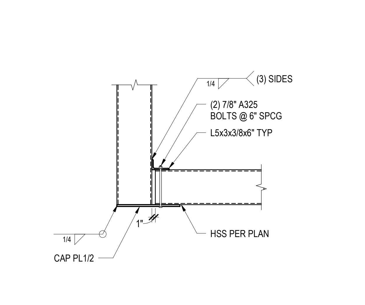
9 SECTION 3/4" = 1'-0"
