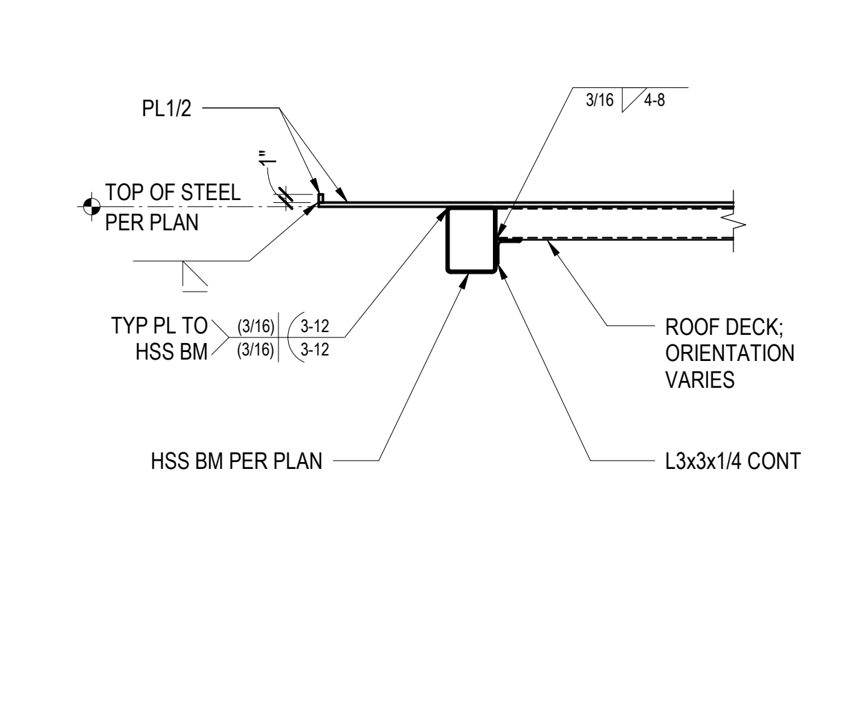
19 SECTION 3/4" = 1'-0"
