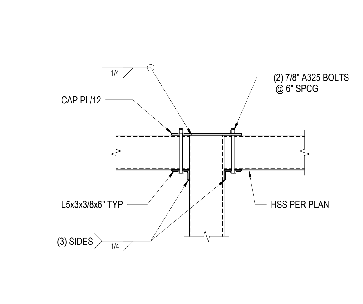
8 SECTION 3/4" = 1'-0"
