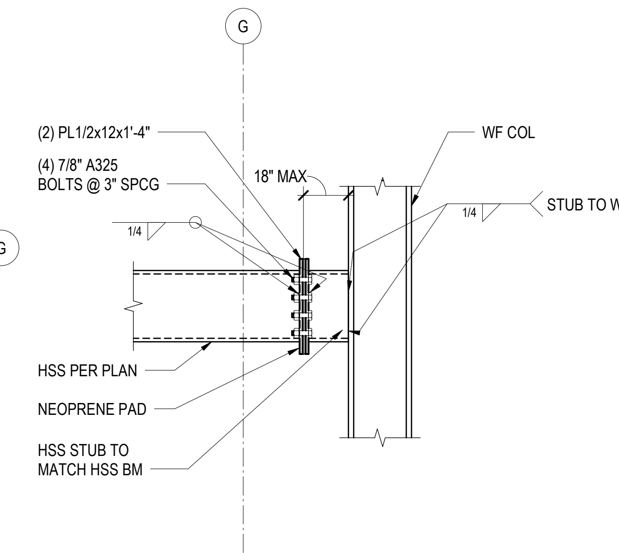
3 SECTION 3/4" = 1'-0"
