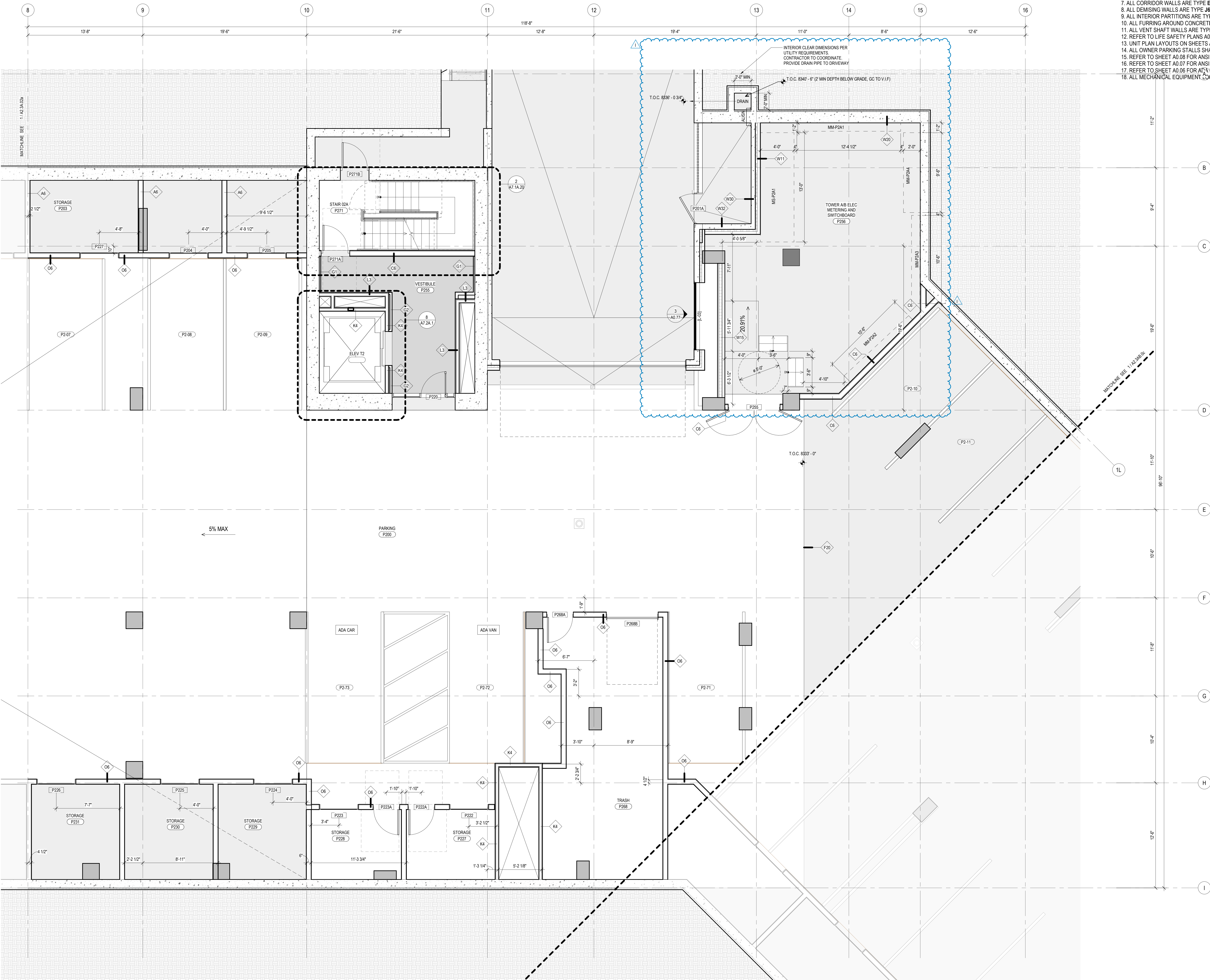
1 TOWER A - LVL P2 - AREA B SCALE: 1/4" = 1'-0"
