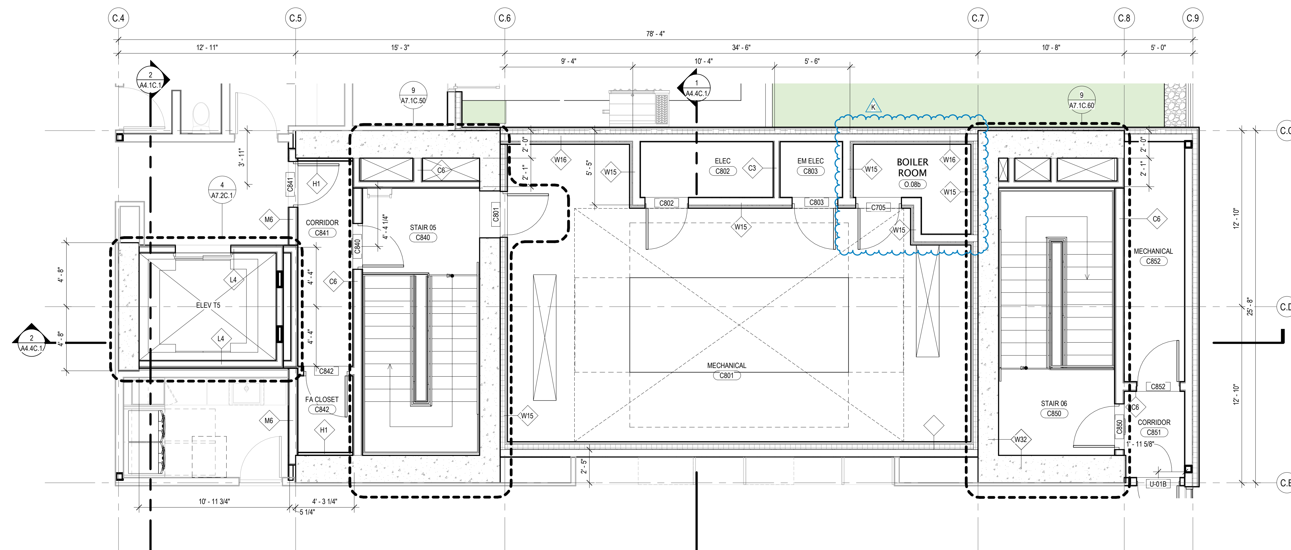
2 TOWER C - LEVEL 8 - CORE SCALE: 1/4" = 1'-0"
