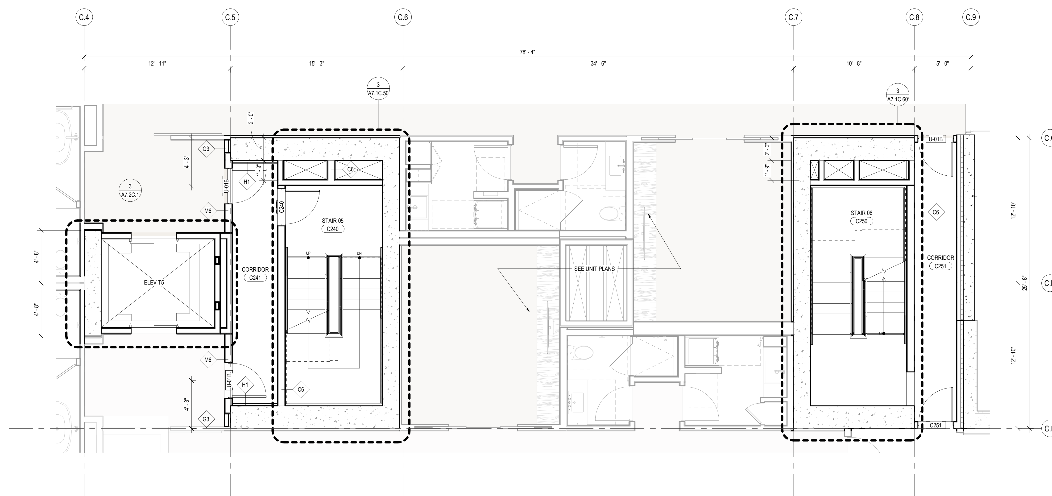
1 TOWER C - LEVEL 2-7 - CORE TYP SCALE: 1/4" = 1'-0"
