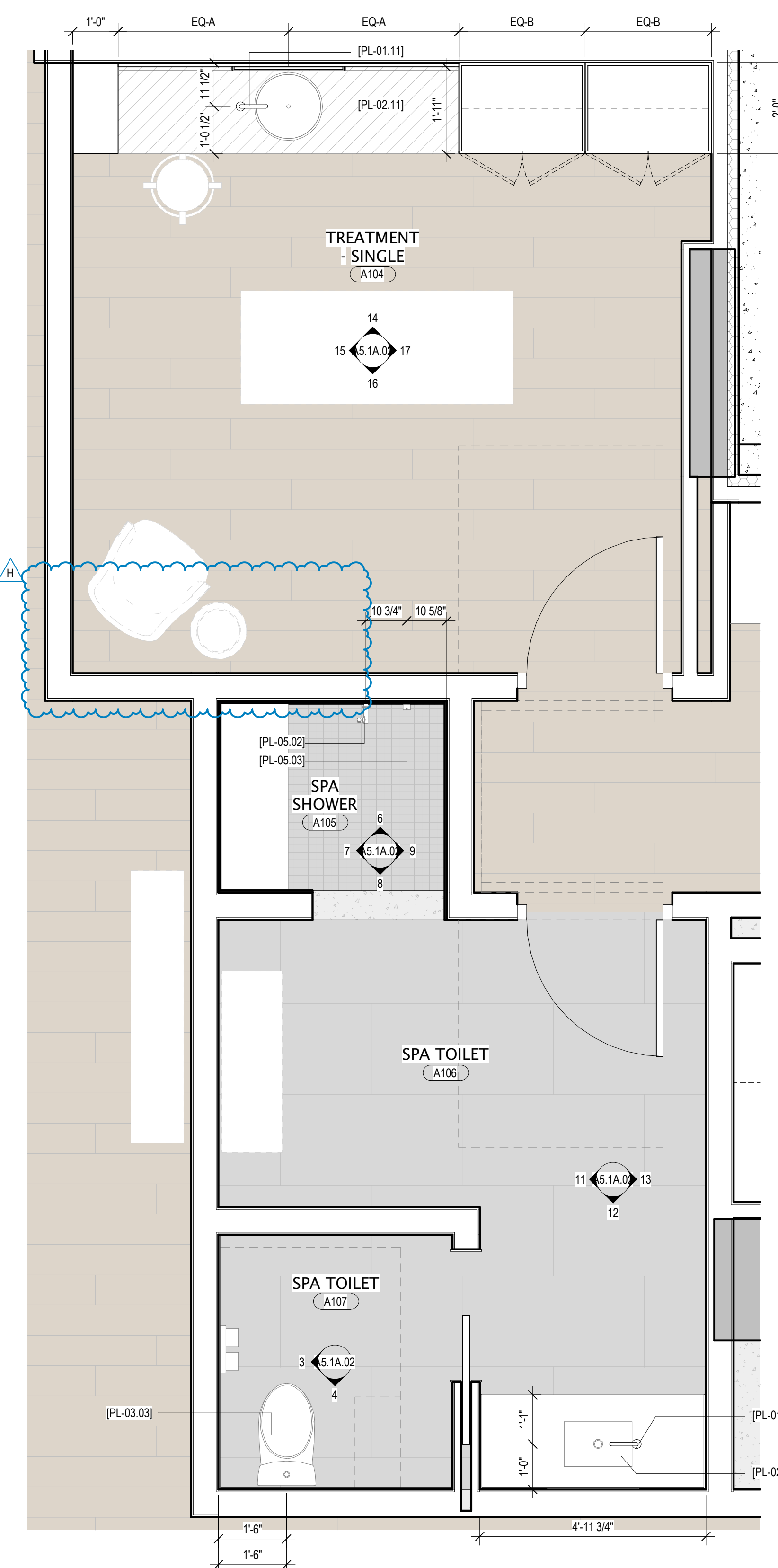
1 ENLARGED PLAN, SPA TREATMENT - SINGLE SCALE: 1/2" = 1'-0"
