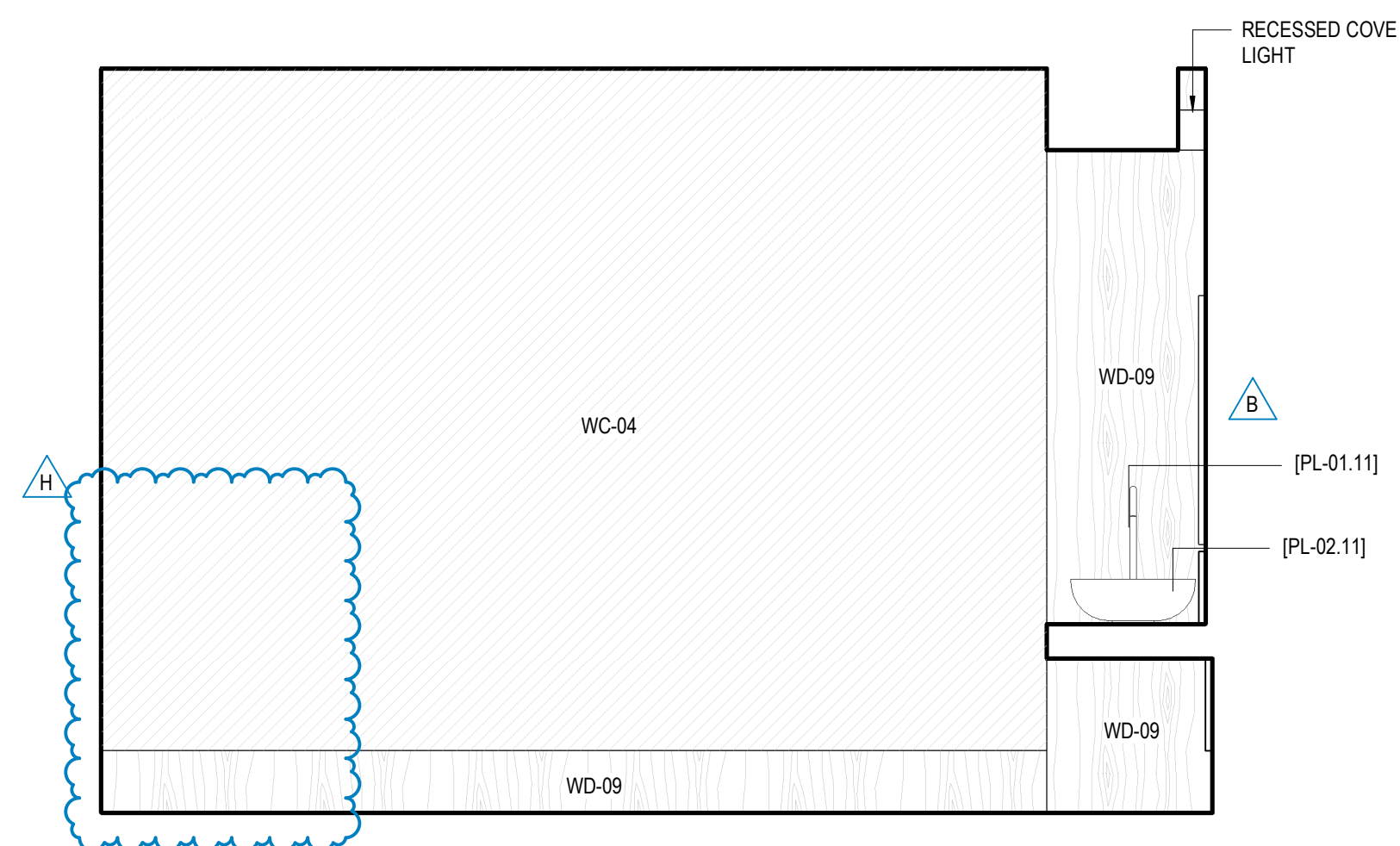
15 SPA TREATMENT SINGLE, 604 - B SCALE: 1/2" = 1'-0"
