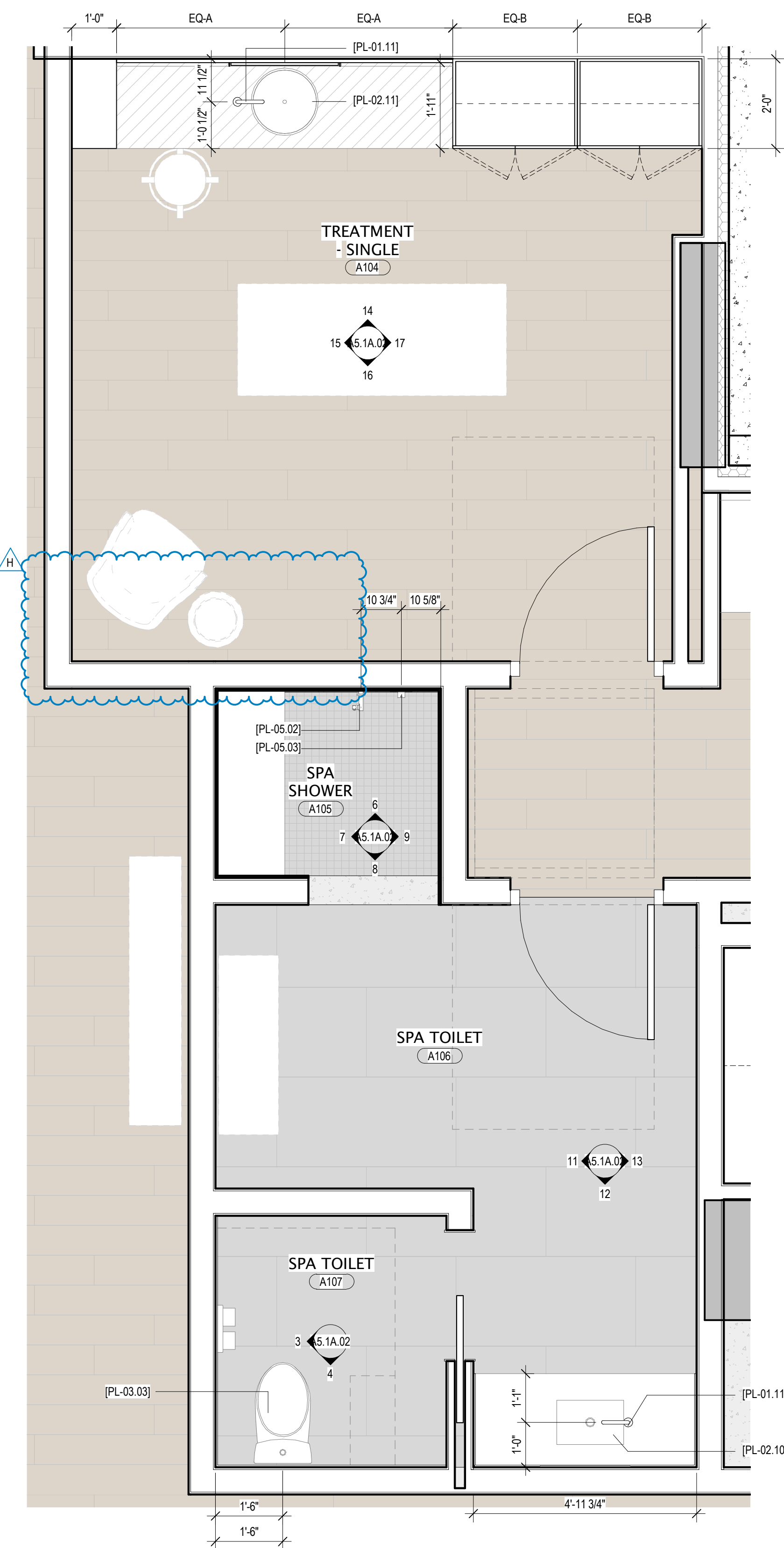
1 ENLARGED PLAN, SPA TREATMENT - SINGLE SCALE: 1/2" = 1'-0"
