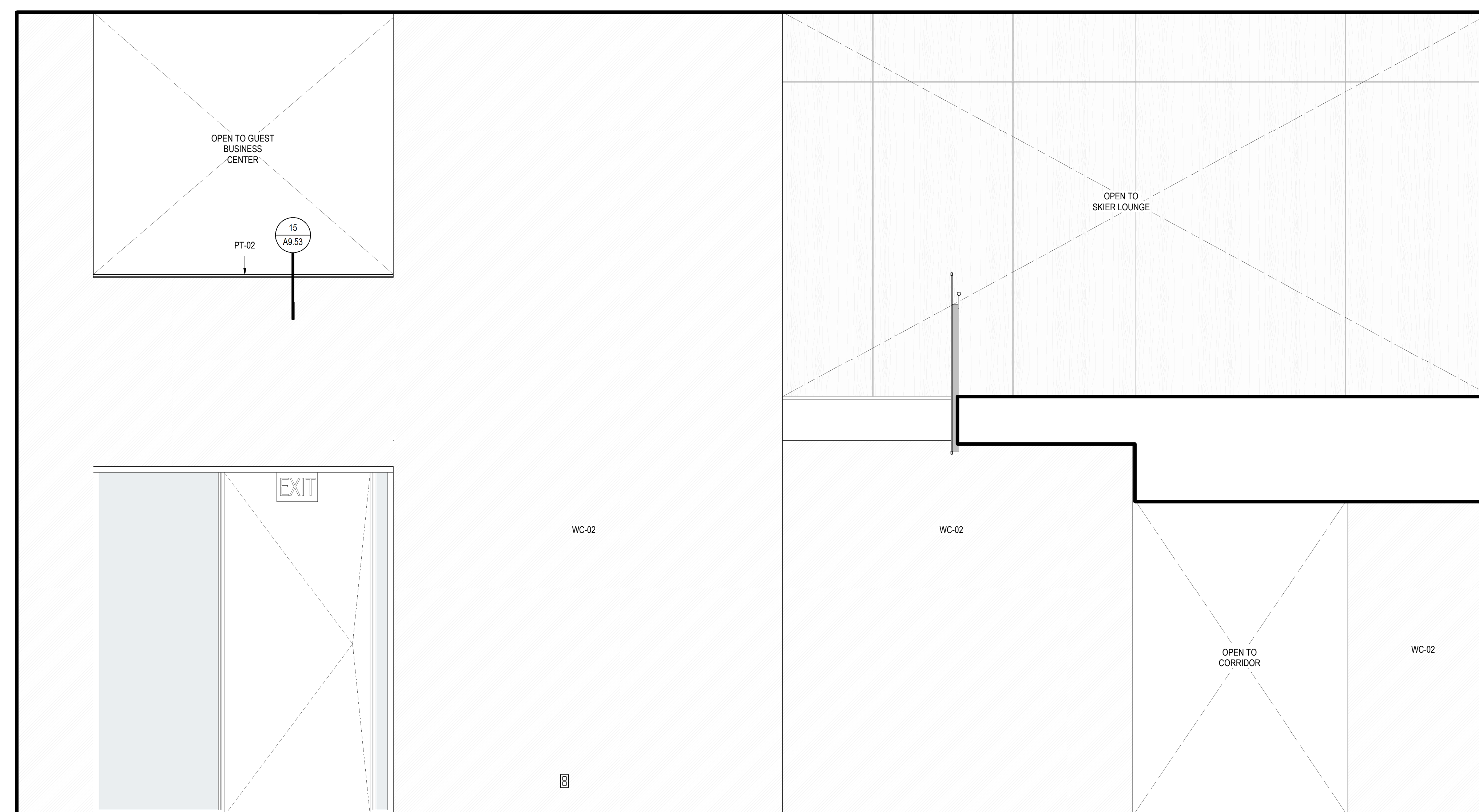
1 ENTRY LOBBY - D SCALE: 1/2" = 1'-0"
