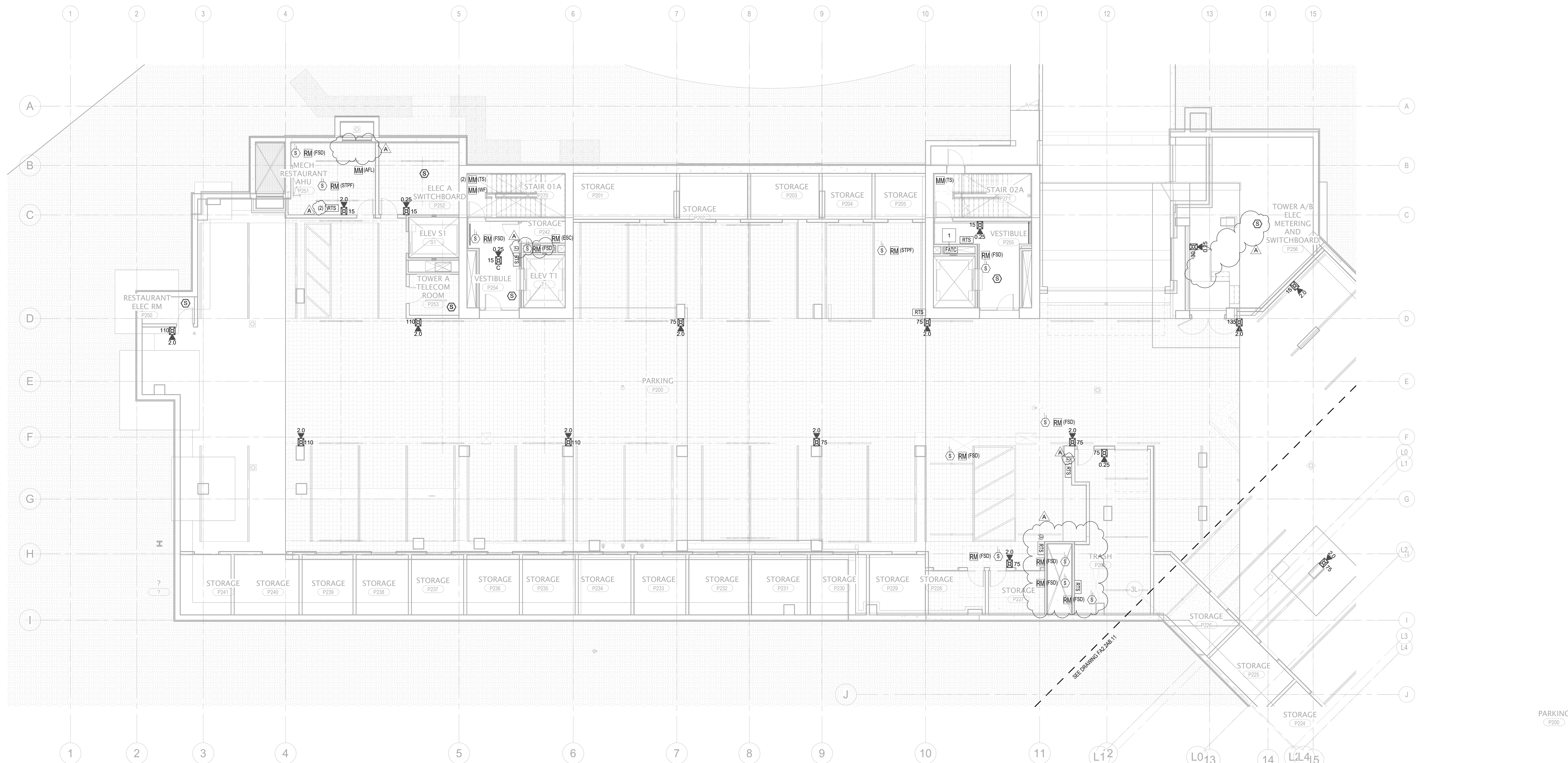
1 TOWER A - PARKING LEVEL 2A - FA 1/8" = 1'-0"
