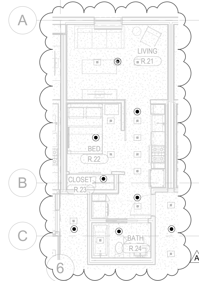
5 ENLARGED PLAN - C - UNIT R 1/8" = 1'-0"
