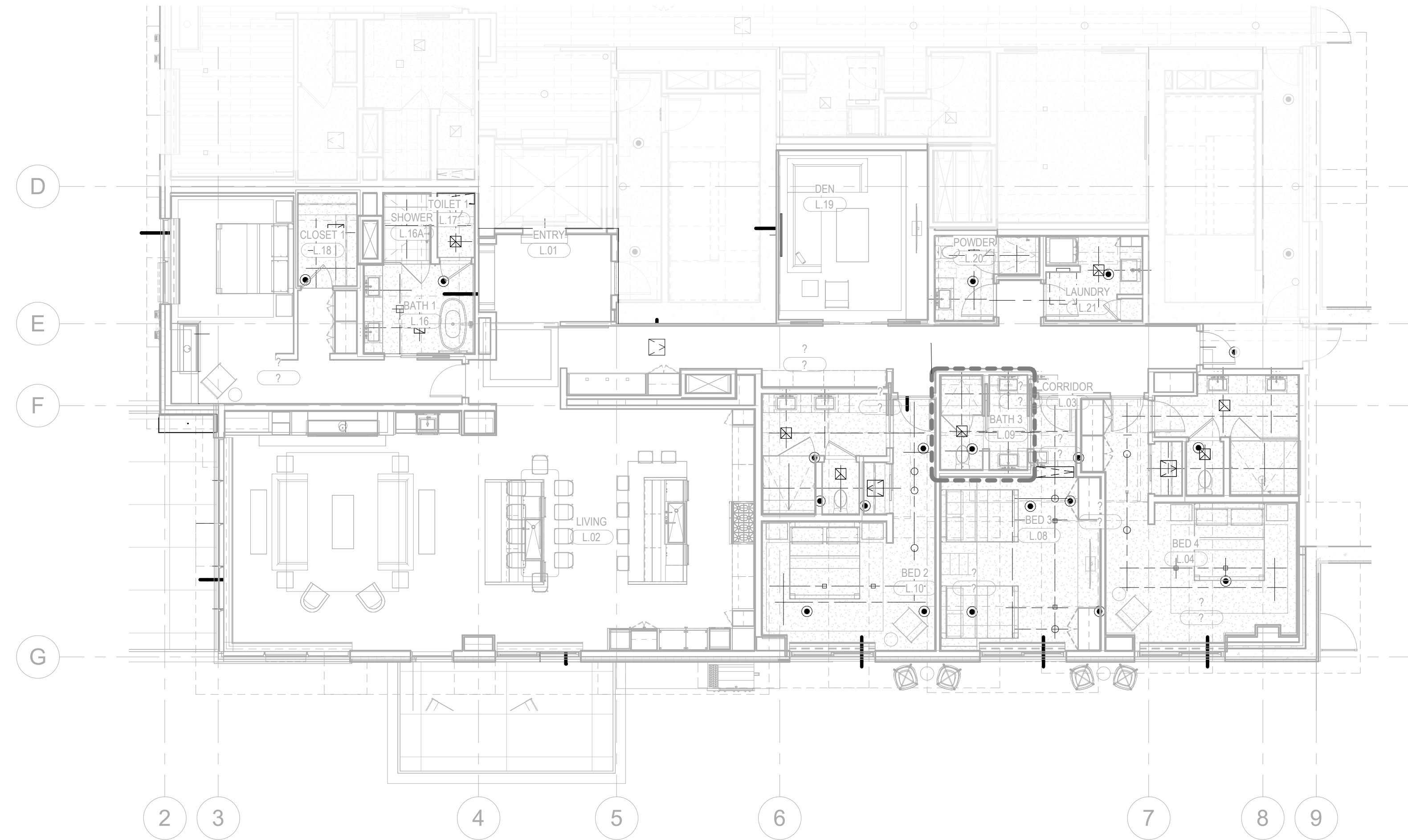
1 ENLARGED PLAN - C - UNIT L 1/8" = 1'-0"
