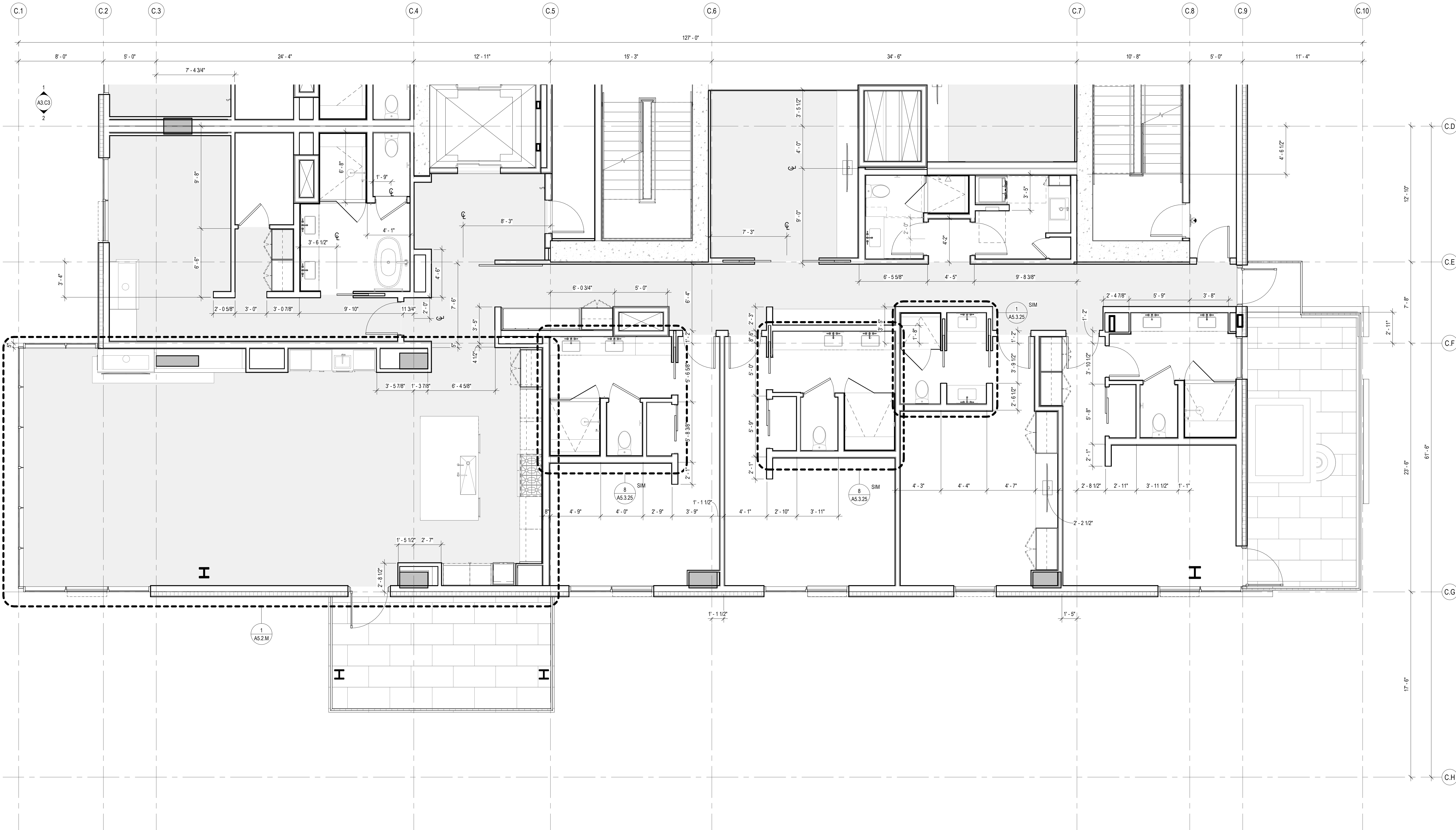
1 TOWER C - UNIT M SOUTH SCALE: 1/4" = 1'-0"
