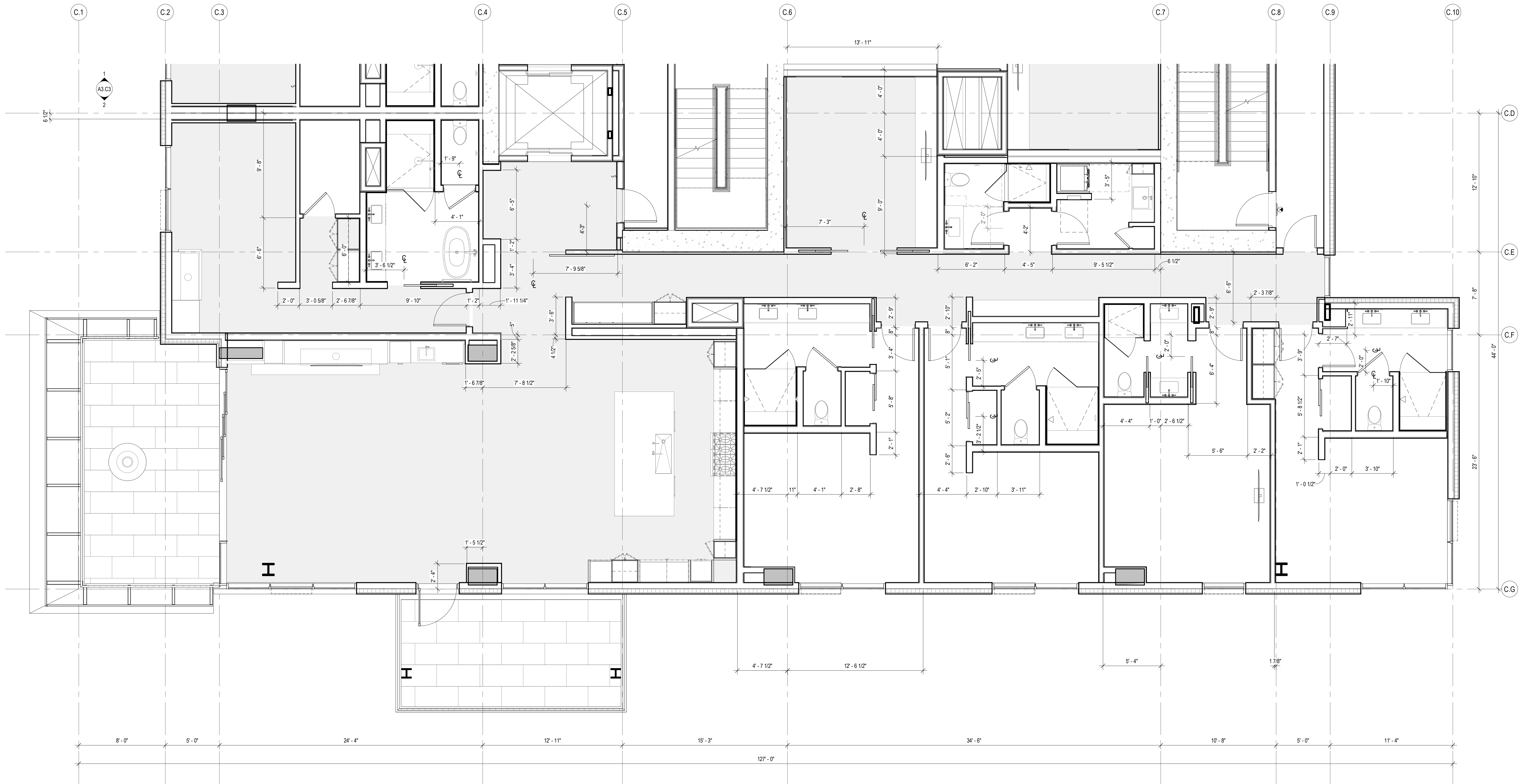
1 TOWER C - UNIT N SOUTH SCALE: 1/4" = 1'-0"
