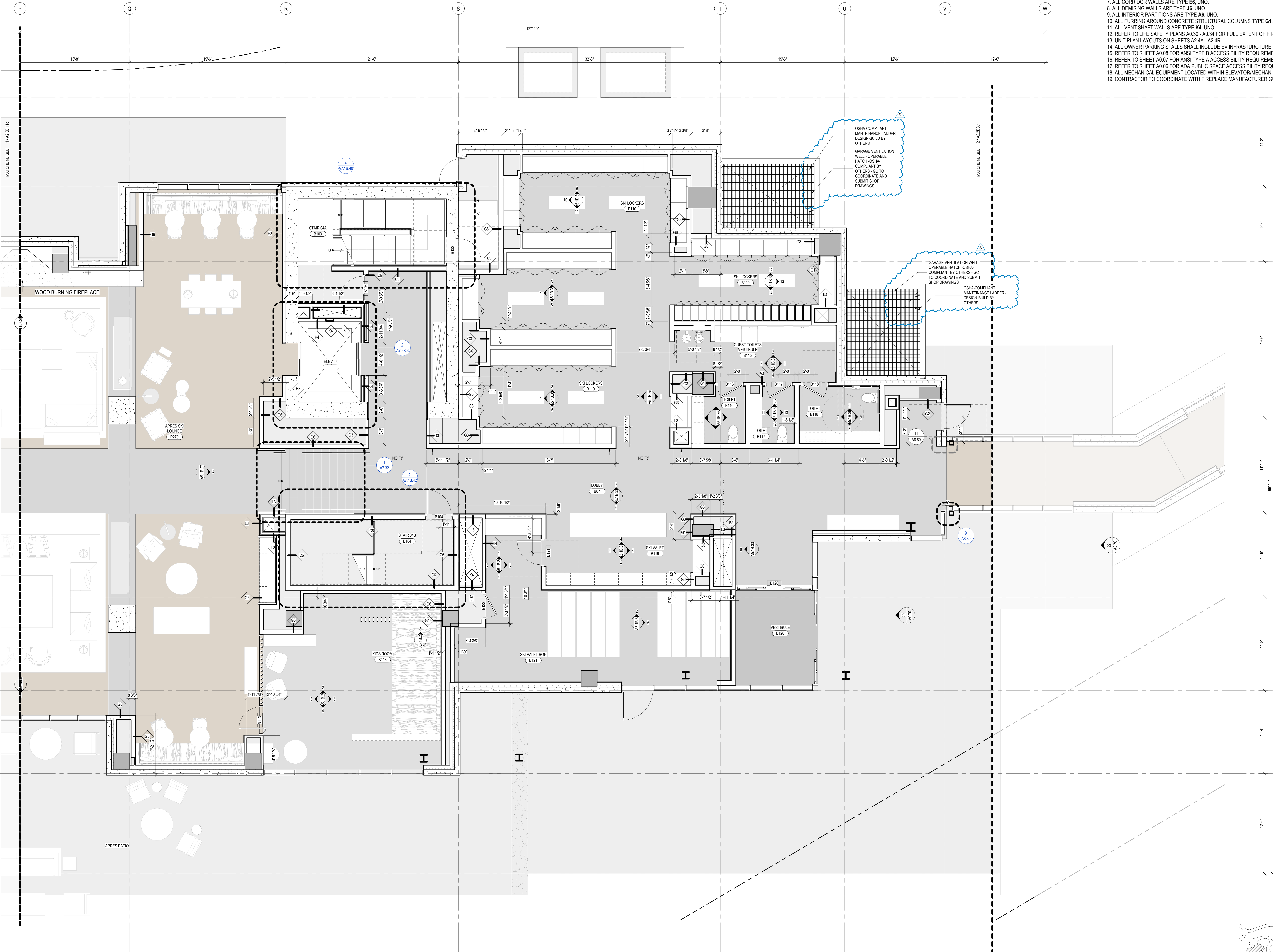
1 TOWER B - LVL 1 - AREA E SCALE: 1/4" = 1'-0"
