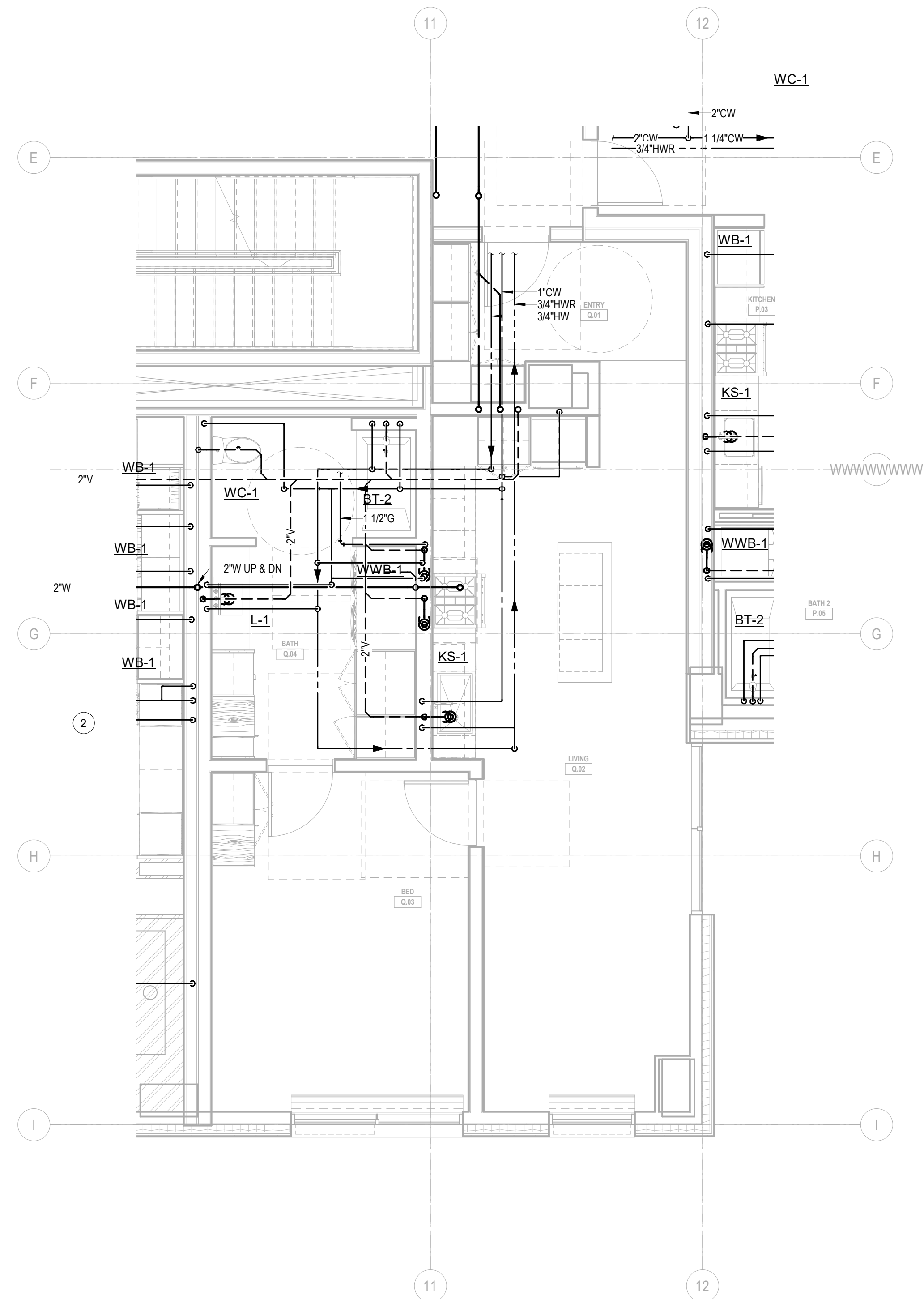
2 ENLARGED PLAN - A/B-UNIT Q SCALE: 1/4" = 1'-0"
