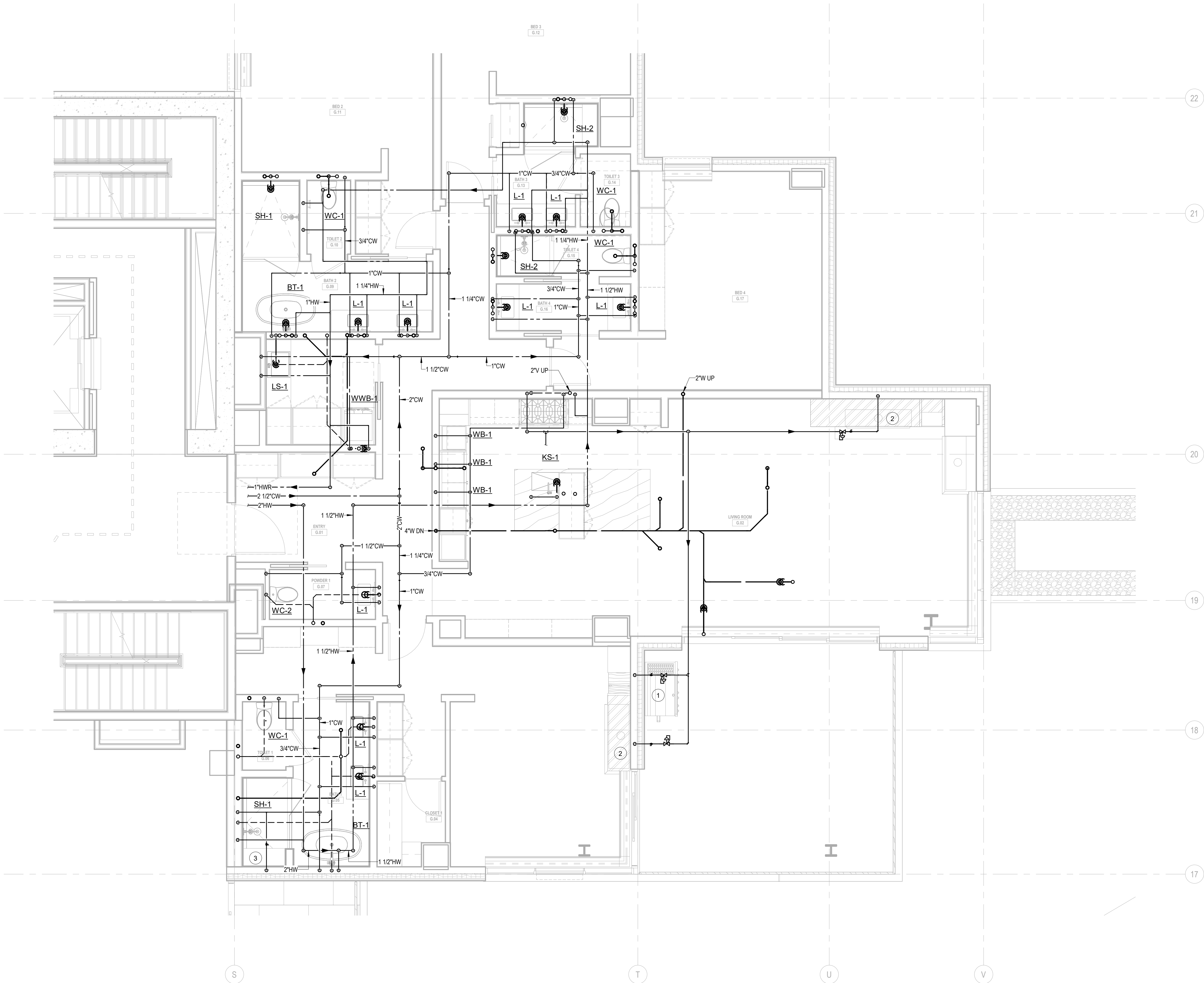
1 ENLARGED PLAN - A/B-UNIT G SCALE: 1/4" = 1'-0"
